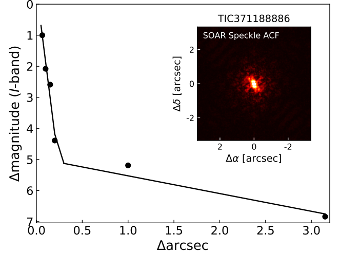
Figure 3. SOAR speckle observations of TOI-2000. The curve is the 5 \sigma detection sensitivity, and the inset is the speckle imaging autocorrelation function (ACF). No companion is detected within the contrast limit.
