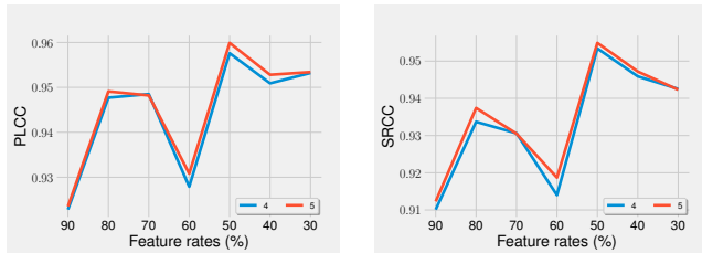
Fig. 6: Effect of feature rate selection on the performance of versions 4 and 5 on OIQA.
