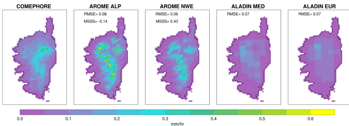
Fig. 7 Amplitude of the summer diurnal cycle of precipitation over Corsica for COMEPHORE, AROME ALP, AROME NWE, ALADIN MED and ALADIN EUR. The corresponding RMSE and the MSSS values are included
