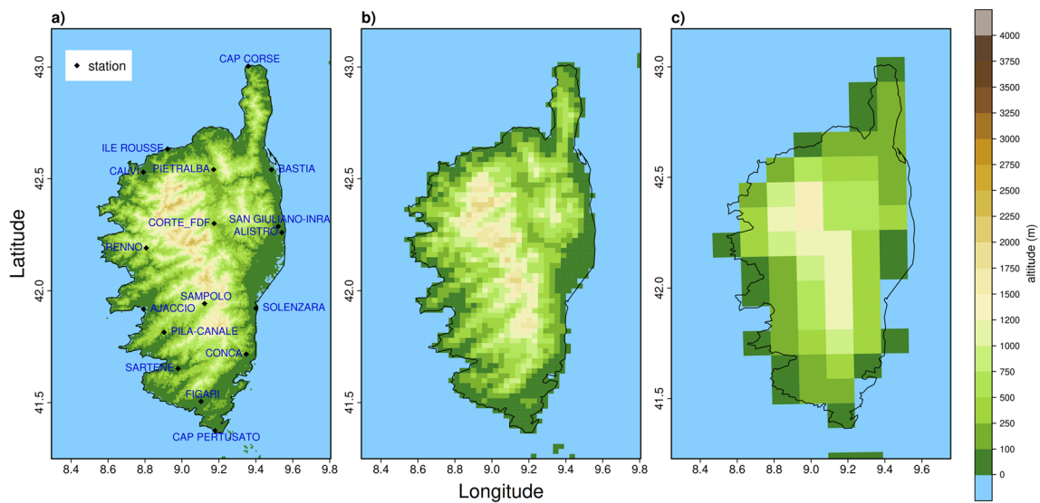
Fig. 1 a Location and name of the 17 weather stations (dots in black) in Corsica. Representation of the orography at different grid resolutions: a land elevation data from the Shuttle Radar Topography Mis-
