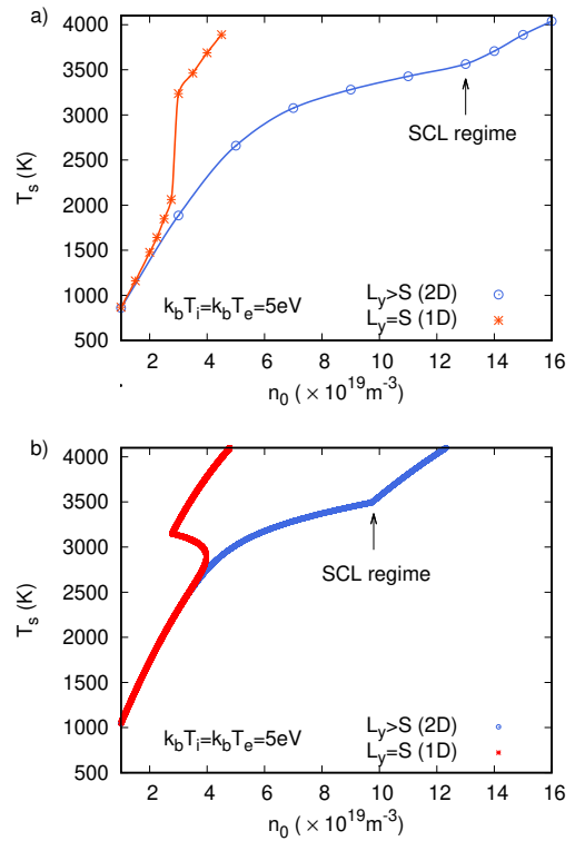
Figure 4: a) Variation of the spot temperature T_s for detached-like divertor conditions with respect to the plasma density n_0 calculated thanks to PIC simulations. b) Spot temperature determined by fluid modeling as presented in section 2.
