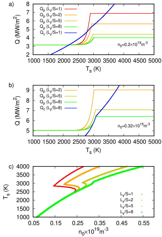
Figure 2: a) Heat flux from the plasma Q_p for different L_y/S ratios and for a plasma density n_0 = 0.2 \times 10^{19} \text{ m}^{-3} . Q_c is the heat flux from the surface. b) Q_p and Q_c for a plasma density n_0 = 0.32 \times 10^{19} \text{ m}^{-3} . c) Spot temperature T_s with respect to the plasma density n_0 for different L_y/S ratios. In all simulations, k_b T_i = k_b T_e = 35 \text{ eV} .
