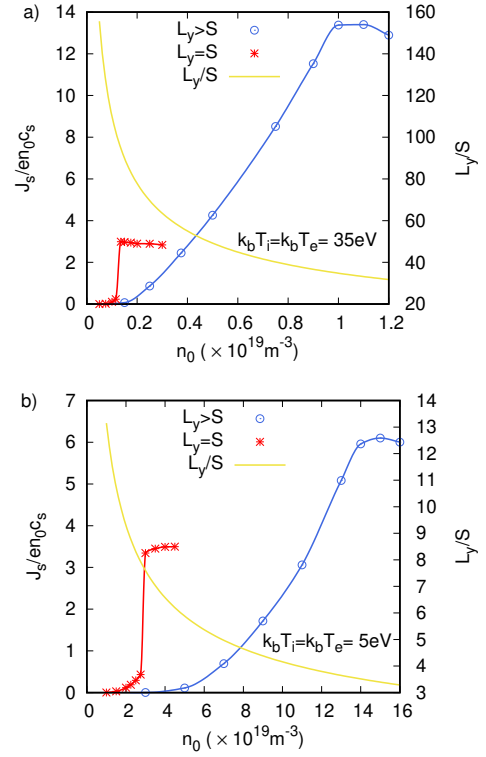
Figure 6: Variation of the thermionic current density J_s for a) attached-like and b) detached-like divertor plasma conditions and for the case L_y = S and L_y = 50\lambda_d > S . The ratio L_y/S plotted in yellow is indicative of the surface available for the return of the plasma electron current in order to achieve quasi-neutrality.
