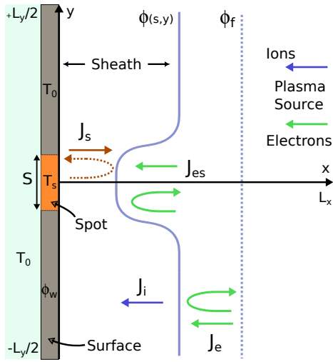
Figure 1: Sketch of the studied plasma bounded by a grounded conductive wall on its left side. The sheath potential profile \phi(s, y) is indicative of what is expected in 2D, with a slightly lower sheath potential at the vertical of the spot than in the rest of the plasma. The profile of \phi_f depicted in the figure is indicative of what is expected for the sheath potential in the absence of thermionic emission.
