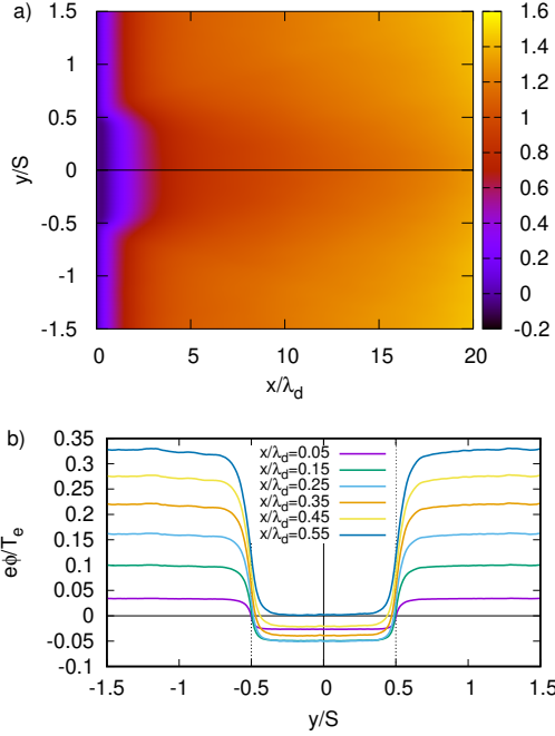
Figure 5: a) Zoom of the 2D density plot of the plasma potential normalized to T_e in the detached-plasma case for n_0 = 15 \times 10^{19} \text{ m}^{-3} . b) Corresponding variation of the normalized potential in the y direction for different abscissas exhibiting the virtual cathode at the spot location.
