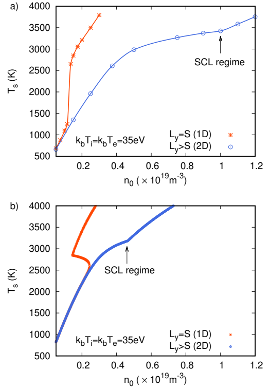
Figure 3: a) Variation of the spot temperature T_s for attached-like divertor conditions with respect to the plasma density n_0 calculated thanks to PIC simulations. b) Spot temperature determined by fluid modeling as presented in section 2.
