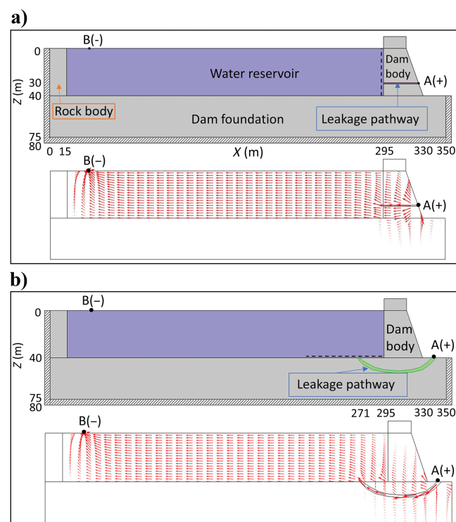
Figure 7. Geometry of the dam body and foundation leakage. (a) Dam model 1: the shaded portion represents the infinite-element domains. Electrode A (+) is located downstream at the leakage outlet, and electrode B (-) is upstream. (b) Dam model 2: the red arrows indicate the current density, which is the maximum at the leakage pathway.
