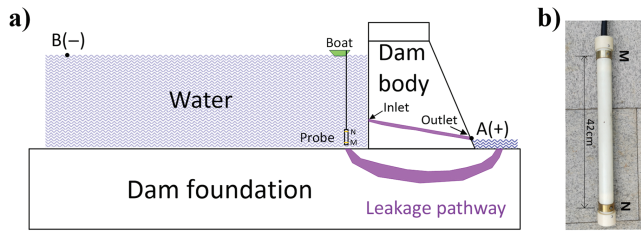
Figure 4. Layout of the electrode array used at the reservoir’s bottom. (a) Cross section of the dam and measurement used to detect leakage inlets using the FFF method. The figure shows two types of leaks, one in the dam body itself and the other in its foundations; A and B denote the current electrodes whereas N and M denote the voltage electrodes. (b) A probe with two ring voltage electrodes to measure the potential difference of the transmitted signal electrical field.
