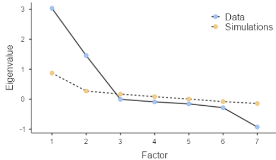
Scree Plot
