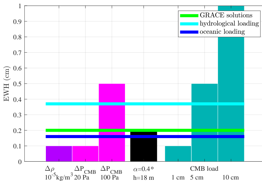
Fig. 2. Uncertainties of degree-2 GRACE solutions (green) and of hydrological (cyan) and oceanic (blue) loading with respect to expected degree-2 surface gravity perturbations by some dynamical core processes: density anomalies and pressure anomalies at the CMB associated with core flows (magenta and pink color), reorientation of the inner core (black) and topographic loading at the CMB for various degree-2 topographic heights (1, 5 and 10 cm) (turquoise). Amplitudes are given in Equivalent Water Height (EWH) in cm.
