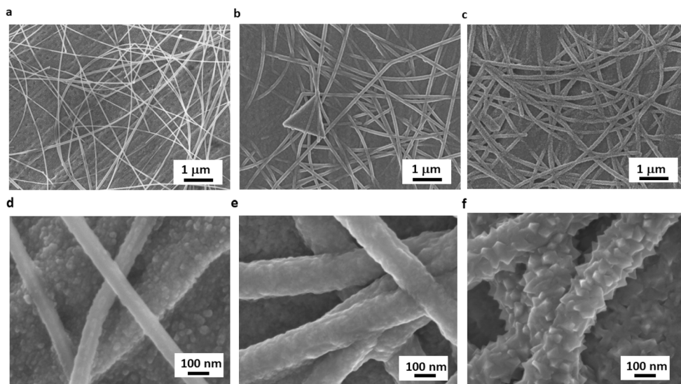
Fig. 3 Morphological analysis of various coatings deposited on Cu sheet. Low and high magnification SEM images of (a and d) bare AgNWs, (b and e) AgNWs@50 nm-thick \text{Cu}_2\text{O} , and (c and f) AgNWs@100 nm-thick \text{Cu}_2\text{O} .
