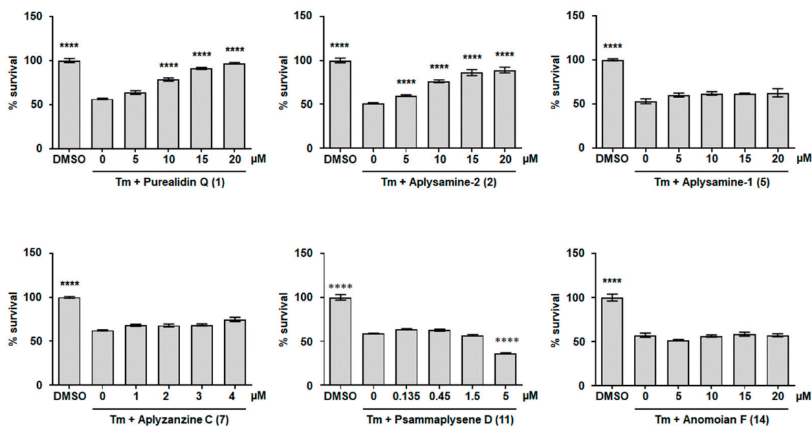
Figure 8. Cytoprotective activity of bromotyrosine derivatives purealidin Q ( 1 ), aplysamine-2 ( 2 ), aplysamine-1 ( 5 ), alyzanzine C ( 7 ), psammaplysene D ( 11 ), and anomoian F ( 14 ) against ER stress. CHO-K1 cells were ER-stressed using 0.45 \mu\text{g}/\text{mL} tunicamycin (Tm) in the presence of the indicated concentrations of the test molecules or DMSO as a negative control. After 24 h of treatment, cell viability was measured by the quantification of the number of live cells using the WST-8 tetrazolium salt. Values are shown relative to the DMSO-treated cells, which was set at a value of 100%. A representative assay including three technical repeats is shown with SD error bars, and each experiment was performed at least three times with similar results. Bar height represents the mean relative to DMSO-treated cells. **** p < 0.0001 one-way ANOVA compared with Tm-treated cells, followed by Dunnett's test.
