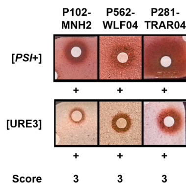
Figure 1. Sponge extracts displaying activity against [PSI+] and [URE3] yeast prions. Yeast cells were spread on a rich agar medium and small sterile filters were then placed on the agar surface, and 2 \mu L of each 10 mg/mL sponge extract was applied to the individual filters. A red halo around the filter on which an extract was loaded indicates that the extract is active against [PSI+] or [URE3] prions, whereas colonies that remain white indicate inactive extracts. Screening scores were attributed according to Table 1.
