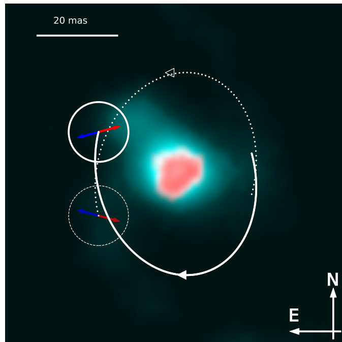
Fig. 9. Composite-colour image with the flux in L band ( 3.60 \mu\text{m} ) displayed in red and flux in N band ( 10.50\text{--}11.50 \mu\text{m} ) shown in blue. The solid white (dashed) circle represents the 3\sigma position prediction at MATISSE epoch for the clockwise (counter-clockwise) orbital motion. The white arcs show the path of the companion around the primary since the last superior conjunction, and the blue (red) arrow represents the sky-projected jet axis for the blueshifted (redshifted) direction.
