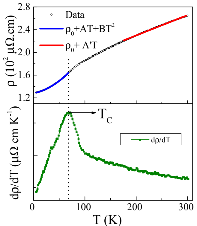
FIG. 9. Temperature dependence of electrical resistivity of FeRuVSi compound in the absence of magnetic fields. The graph exhibits metal-like resistivity behavior throughout the measured temperature region 5-300 K, with a noticeable change in slope near the transition temperature ( T_C ).
