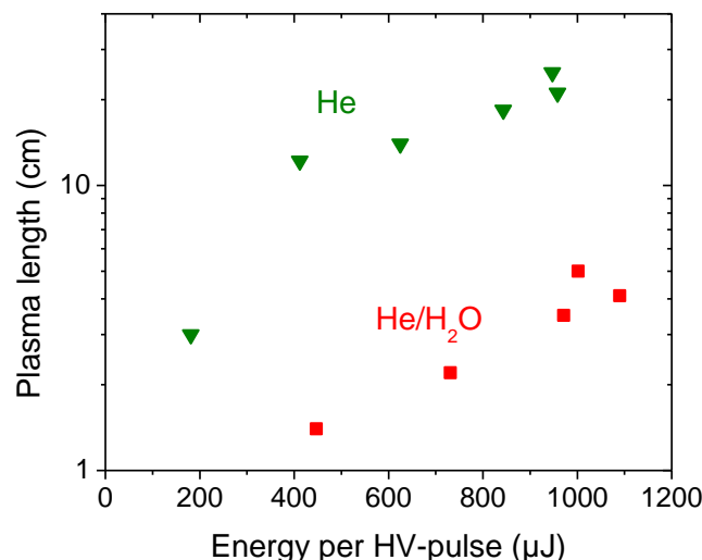
Figure 3 – Plasma length in the micro-capillary tube for pure helium and for the mixture He/H 2 O(2.5%).
