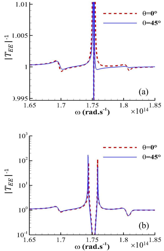
Figure 7. Resonance frequency for a dimer of InSb particles (radius R = 50 \text{ nm} ) separated by a distance 6 = 6R (a) in vacuum and (b) on a transparent substrate ( \epsilon_{sub} = 4 ) under the action of an external magnetic field of magnitude H_{ext} = 5T making an angle \theta with the z axis.
