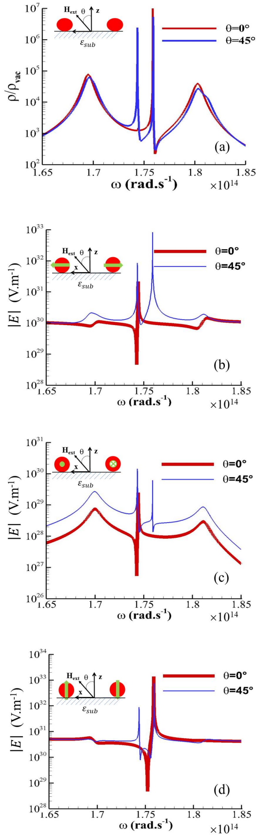
Figure 6. (a) LDOS in the same system as in Fig.5 ( H_{ext} = 5T ) in presence of a substrate ( \epsilon_{sub} = 4 ). (b)-(c) and (d) Magnitude of electric field radiated by two permanent (normalized) dipoles oriented in opposite direction along the x , y and z axis, respectively.
