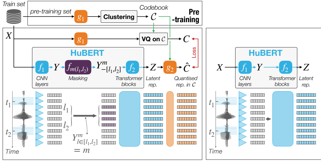
(a) HuBERT training
