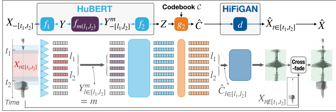
(c) HuBERT-based inpainting pipeline – informed case (inference)
