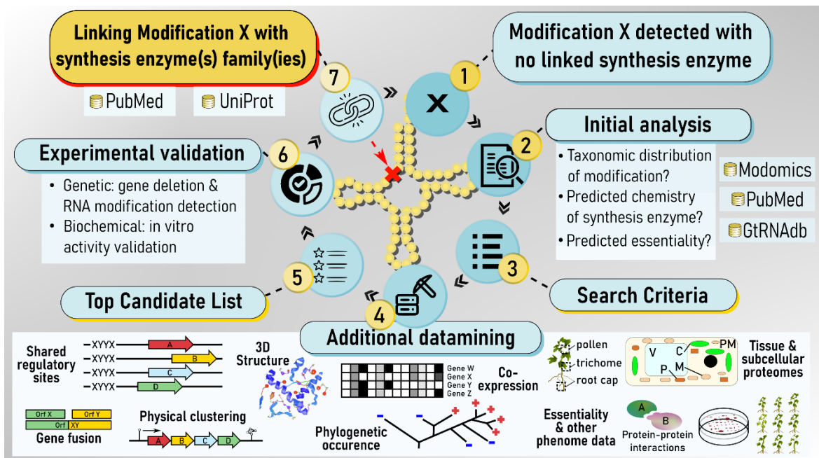
Figure 2. Comparative genomic pipeline to identify missing tRNA modification genes. The search starts by mapping tRNA modifications to known enzymes to identify globally or locally missing enzymes (1). After an initial datamining step (2) to define search criteria (3), a combination of in silico tools that integrate different types of in silico and omics data (4) can be used to generate a candidate list (5) that will be experimentally validated (6) before deposition in databases as a novel tRNA modification genes (7). Modomics is a database of RNA modification. GtRNAdb is a Genomic tRNA database.
