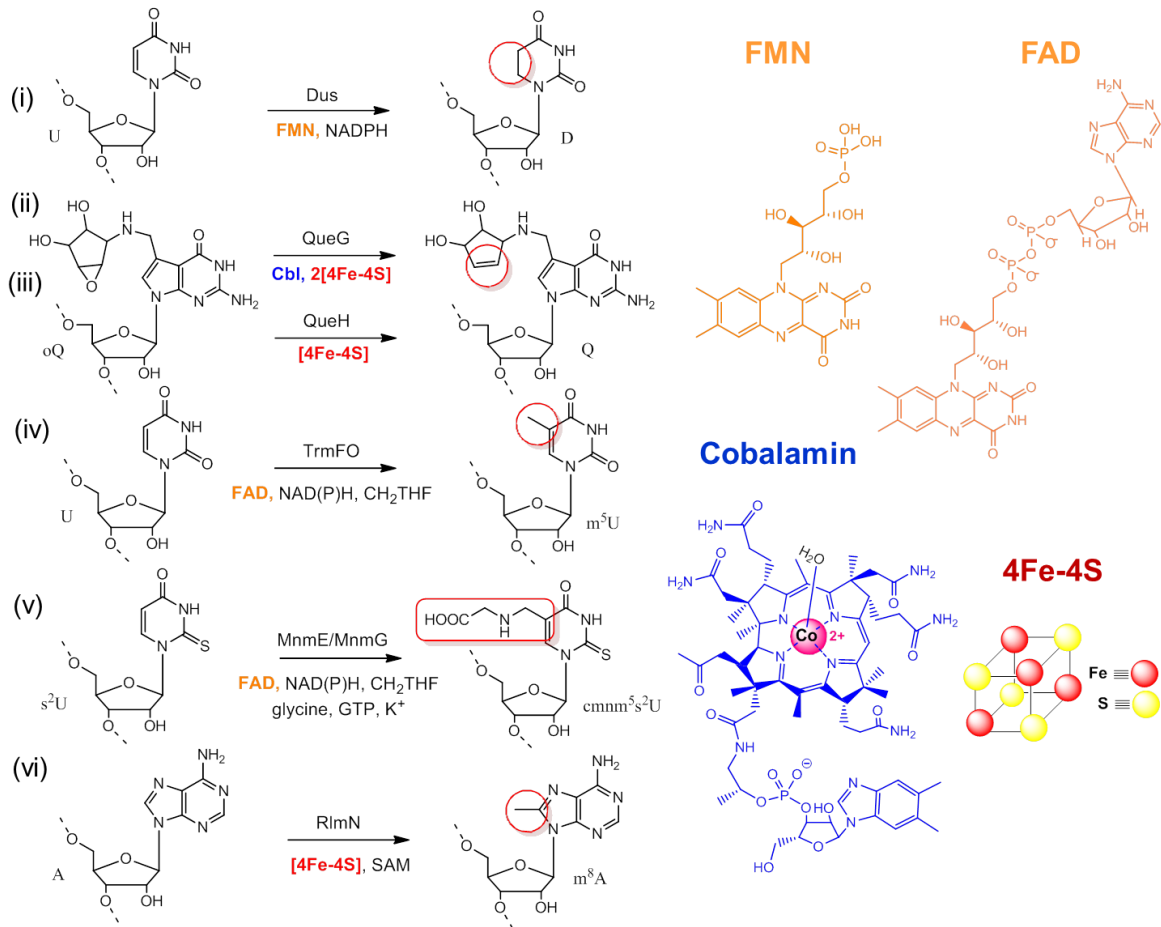
Figure 1. RNA modifications dependent on redox coenzymes. Left side: biosynthetic RNA modifications for: (i) the reduction of uridine to dihydrouridine (D) catalyzed by the dihydrouridine synthases (Dus), (ii) the \text{o}^{\text{Q}} reduction to Q by QueG and QueH, (iii) the reductive methylation of uridine into \text{m}^5\text{U} by TrmFO, (iv) the carboxymethylaminomethylation of uridine into \text{cmnm}^5\text{U} catalyzed by MnmE/mnmG complex (v) the methylation of adenine to \text{m}^8\text{A} by RlmN. (vi) The chemical groups of each modification are boxed in red and the respective enzyme(s) that catalyze each reaction are indicated. Right side: Biochemical coenzymes used for RNA modifications: flavins (FMN and FAD) in orange, cobalamin (Cbl) in blue and its metal in magenta, while the cubic 4Fe-4S cluster is represented with Fe atoms in red and sulfur in yellow.
