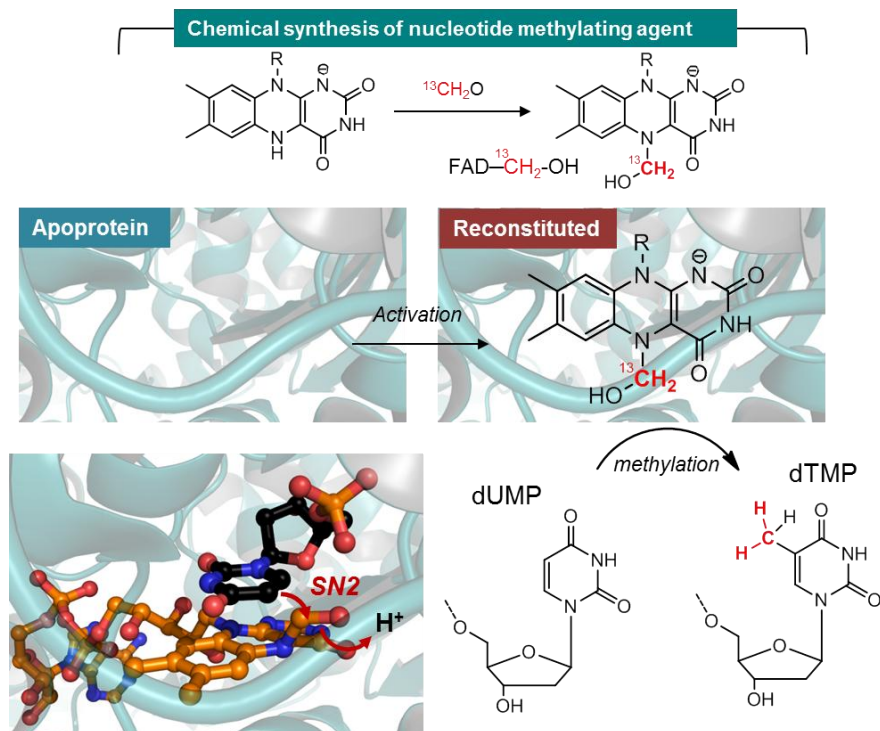
Figure 5. Formaldehyde shunt to activate an apoprotein of a folate and flavin-dependent methyltransferase. FADH - (reduced flavin), obtained by the reduction of oxidized FAD with dithionite, activates 13 C-labeled formaldehyde via the N5 of the isoalloxazine to give an air-labile flavin carbinolamine. The latter can be reconstituted in an apoprotein version of Thermus thermophilus thymidylate synthase (ThyX) that uses flavin and folate to catalyze the reductive methylation of the uracil C5 of dUMP to dTMP. This reaction is similar to that of TrmFO or RlmFO. Once reconstituted with the synthetic carbinolamine under anaerobic conditions, the methyltransferase is active and can readily methylate dUMP. The crystallographic structure of this carbinolamine intermediate (orange) is shown in complex with dUMP (black) by structural alignment. Once activated, the C5 uracil of the substrate attacks the electrophilic methylene of the carbinolamine allowing its transfer from the flavin to dUMP.
