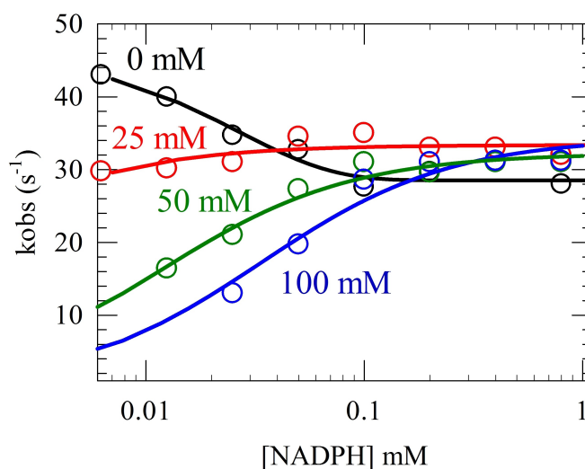
Figure 4. Effect of MgCl_2 on the kinetics of reduction of hAdxR with NADPH. Dependence of the observed rate constant for hAdxR reduction ( k_{obs} ) as a function of NADPH determined at 450 nm in the presence of different MgCl_2 concentrations as indicated on each curve.
