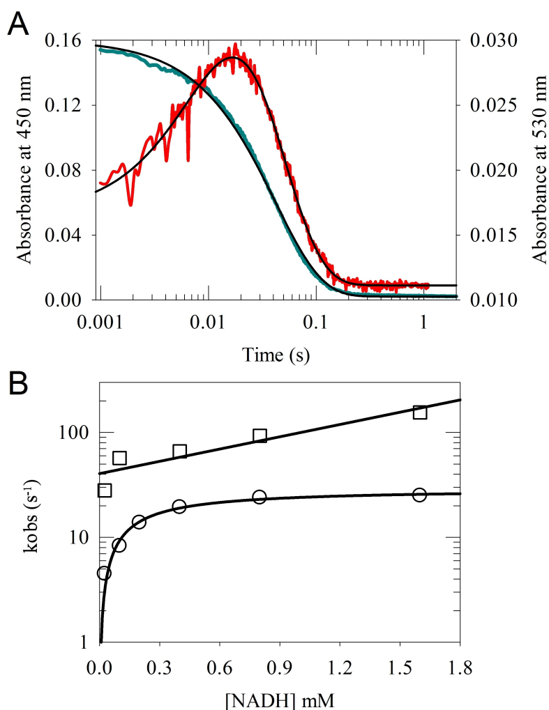
Figure 2. Kinetics of reduction of hAdxR by NADH. (A) Kinetic traces of hAdxR (15 \mu M) reduction by NADH recorded by following the absorbance at 450 nm (left axis, green) and 530 nm (right axis, red). (B) Dependence of the observed rate constant for hAdxR reduction ( k_{obs} ) as a function of NADH determined at 450 nm (circle) and 530 nm (square).
