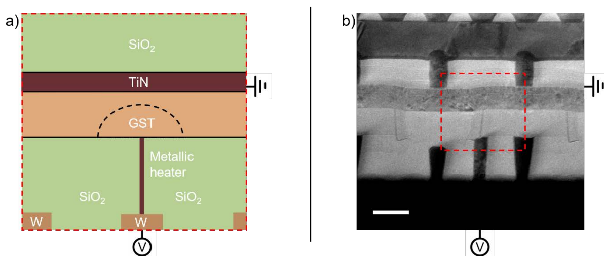
Figure 1. a) Schematic representation of a PCM in a Wall architecture and b) PCM cell studied by operando holography. The dotted red rectangle corresponds to the area studied below. Scale bar is 100 nm.
