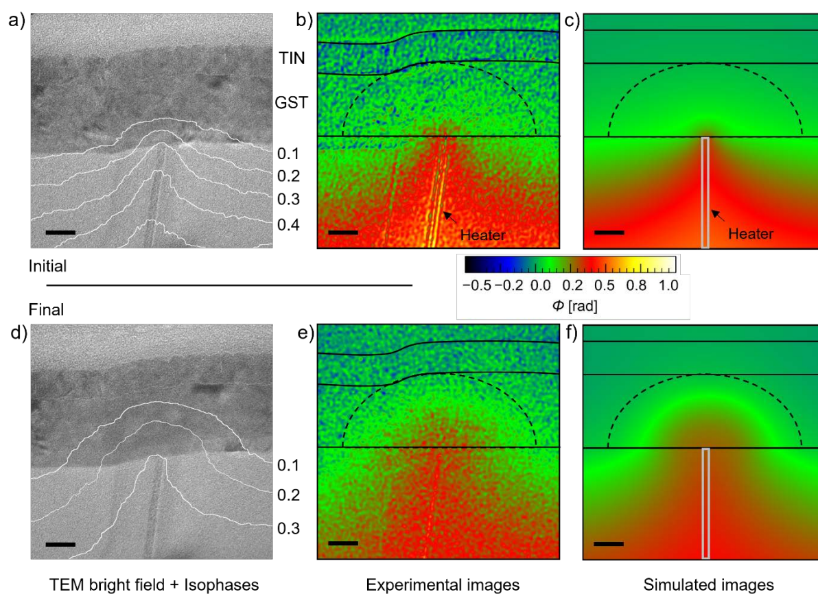
Figure 2. Conventional bright-field TEM image, Initial state (a), Final state (d) with isophase contours (values on the right) extracted from experimental phase maps, Initial (b), Final (e). Simulated phase maps, Initial (c), Final (f). In dotted line the dome-like shape where the phase change occurs. Scale bars are 20 nm.
