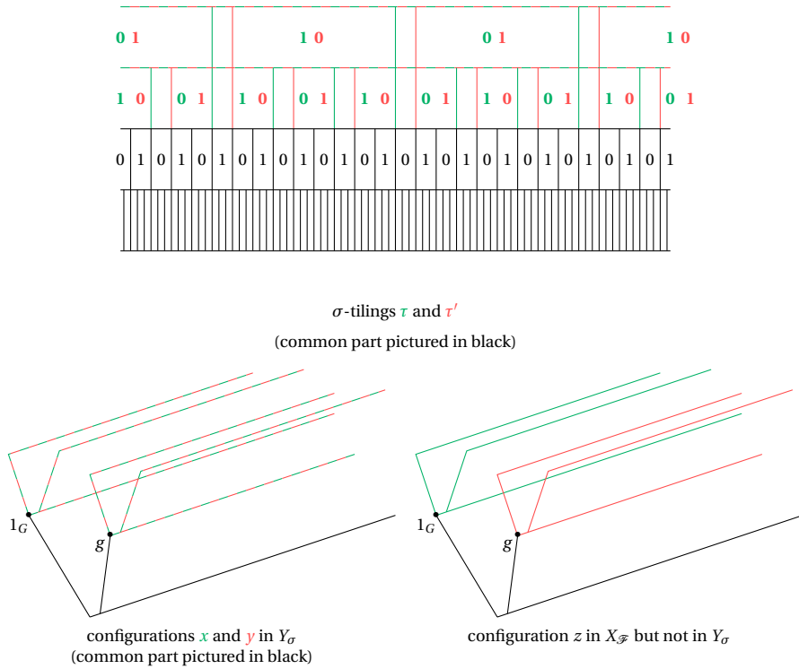
Figure 5. The substitution given by \sigma(0) = 010 and \sigma(1) = 101 is not recognizable, hence the subshift Y_\sigma is not SFT.
