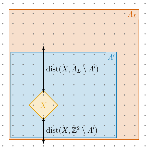
Figure 2: Sketch of the two distances used in Definition 1. If the Hamiltonian satisfies local indistinguishability in the bulk, the bound (6) decays in the distance to the boundary of \Lambda' (in \mathbb{Z}^2 ). While local indistinguishability everywhere also gives a good estimate if X is close to the boundary of \Lambda' as long as the boundaries of \Lambda' and \Lambda_L coincide in that region.
