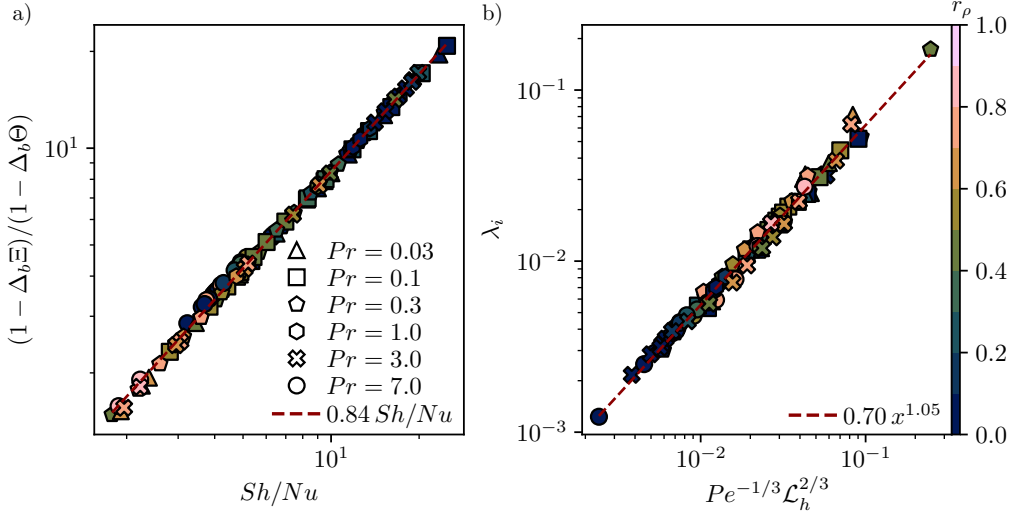
Figure 6: (a) (1 - \Delta_b \Xi)/(1 - \Delta_b \Theta) as a function of Sh/Nu . (b) Thickness of the inner boundary layer as a function of Pe^{-1/3} L_h^{2/3} derived in Eq. (3.10). In each panel, the result of the linear regression is shown with a dashed line.
