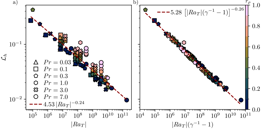
Figure 7: (a) Horizontal lengthscale \mathcal{L}_h (Eq. 2.19) as a function of |Ra_T| . (b) \mathcal{L}_h as a function of |Ra_T|(\gamma^{-1} - 1) . In both panels, the dashed lines correspond to power law fits.
