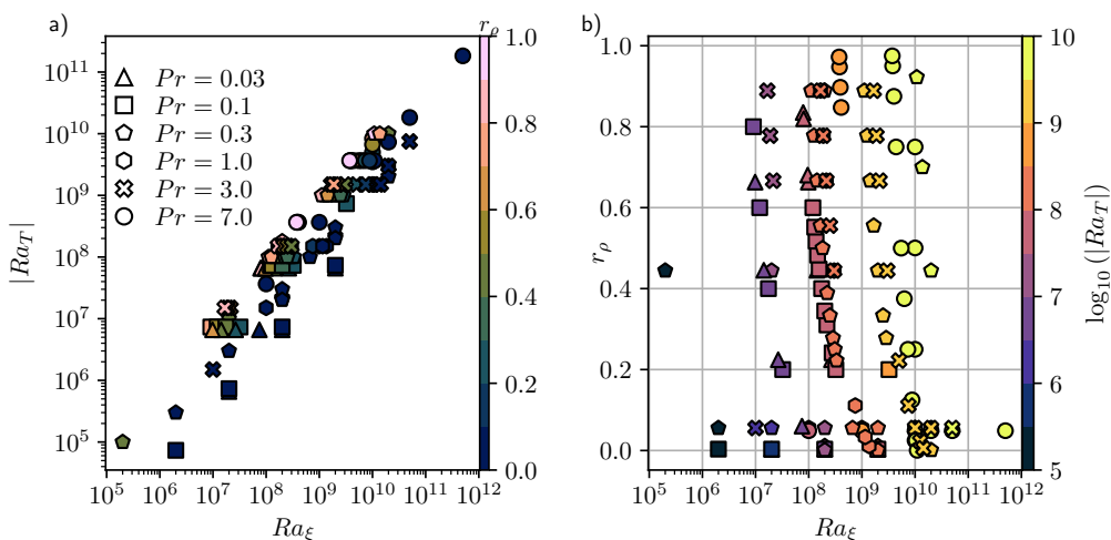
Figure 1: (a) Normalised density ratio r_\rho in the thermal Rayleigh number |Ra_T| - chemical Rayleigh number Ra_\xi plane for the 123 simulations performed for this study. (b) \log_{10}(|Ra_T|) in the Ra_\xi - r_\rho plane for the same simulations. Markers reflect the value of Pr .
