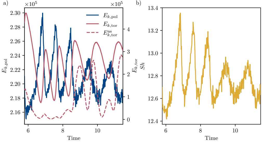
Figure 19: (a) Time evolution of the poloidal kinetic energy (solid blue), the toroidal kinetic energy (solid red), and the axisymmetric toroidal energy (dashed red) for a simulation performed with Ra_T = -10^9 , Pr = 0.3 , Le = 10 , and R_\rho = 4 (simulation 39 in Tab. 3). (b) Time evolution of Sh for that simulation, that is represented with the white star with a yellow rim in Fig. 16.
