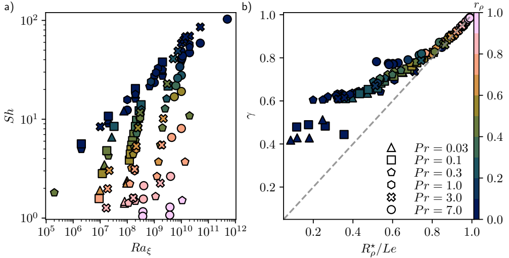
Figure 9: (a) Sherwood number Sh as a function of Ra_\xi . (b) Flux ratio \gamma as a function of R_\rho^*/Le . The dashed line corresponds to the first bisector \gamma = R_\rho^*/Le .
