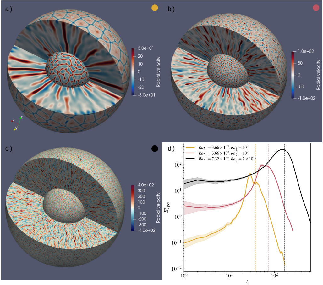
Figure 3: (a-c) Three-dimensional renderings of the radial velocity for three simulations carried out using R_\rho = 1.1 , Pr = 7 and Le = 3 , and Ra_\xi = 10^8 , 10^9 , and 2 \times 10^{10} (simulations 123, 118 and 103 in Tab. 3), for (a), (b) and (c), respectively. Inner and outer spherical surfaces correspond to r_i + 0.03 and r_o - 0.04 , respectively. (d) Poloidal kinetic energy spectra as a function of spherical harmonic \ell for these three simulations. Dashed vertical lines correspond to the average spherical harmonic degree \ell_h (see Eq. 2.19), of value 39, 75 and 166, for Ra_\xi = 10^8 , 10^9 , and 2 \times 10^{10} .
