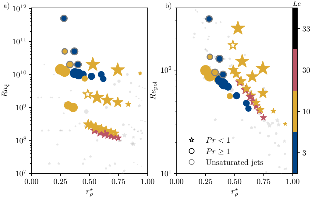
Figure 16: (a) Location of the 123 simulations computed in this study in the (r_\rho^*, Ra_\xi) plane. (b) Same in the (r_\rho^*, Re_{\text{pol}}) plane. Stars and discs denote Pr < 1 and Pr \geq 1 , respectively. Grey symbols correspond to models without jets. Conversely, symbols corresponding to simulations with single or multiple jets according to the criterion (4.1) are colored according to the value of the Lewis number Le . Symbol size is proportional to Re_{\text{tor}}^1 / Re_{\text{pol}} , where Re_{\text{tor}}^1 is the Reynolds number constructed from the spherical harmonic degree \ell = 1 component of the toroidal flow. The 5 simulations with jets whose symbol has a grey rim were not integrated for a long enough time to witness the possible merging of their multiple jets, which may lead to an underestimation of Re_{\text{tor}}^1 / Re_{\text{pol}} . The white star with a yellow rim corresponds to the simulation further discussed in Fig. 19.
