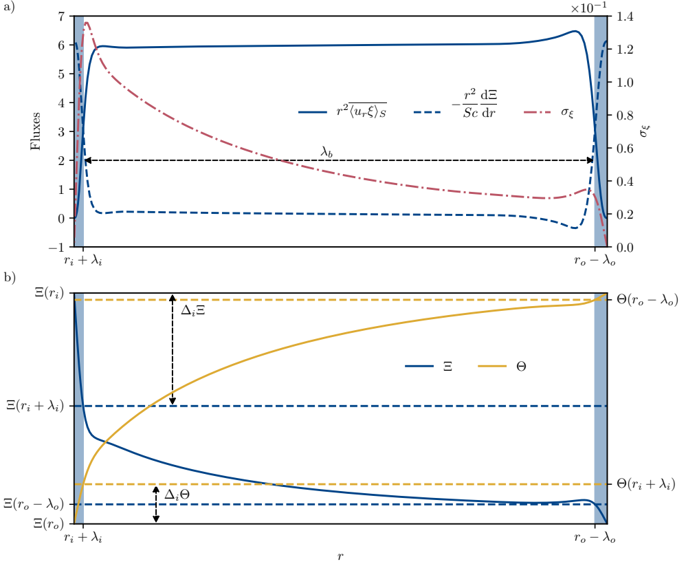
Figure 2: (a) Time-averaged radial profiles of convective and diffusive compositional fluxes, expressed by r^2 \overline{\langle u_r \xi \rangle_S} and -r^2 Sc^{-1} d\Xi/dr respectively (see Eq. 2.13), for a simulation with |Ra_T| = 3.66 \times 10^7 , R_\rho = 1.1 , Pr = 7 , and Le = 3 (simulation 123 in Tab. 3). The radial profile of the variance of composition \sigma_\xi is represented by a dash-dotted line. (b) Time-averaged radial profiles of composition (solid blue line) and temperature (solid mustard line). Horizontal dashed lines highlight the values of composition and temperature at the edges of the convective bulk. \Delta_i \Xi ( \Delta_i \Theta ) is the composition (temperature) drop across the inner boundary layer. The blue-shaded areas highlight the inner and outer chemical boundary layers, of thickness \lambda_i and \lambda_o , respectively, while the convective bulk has thickness \lambda_b .
