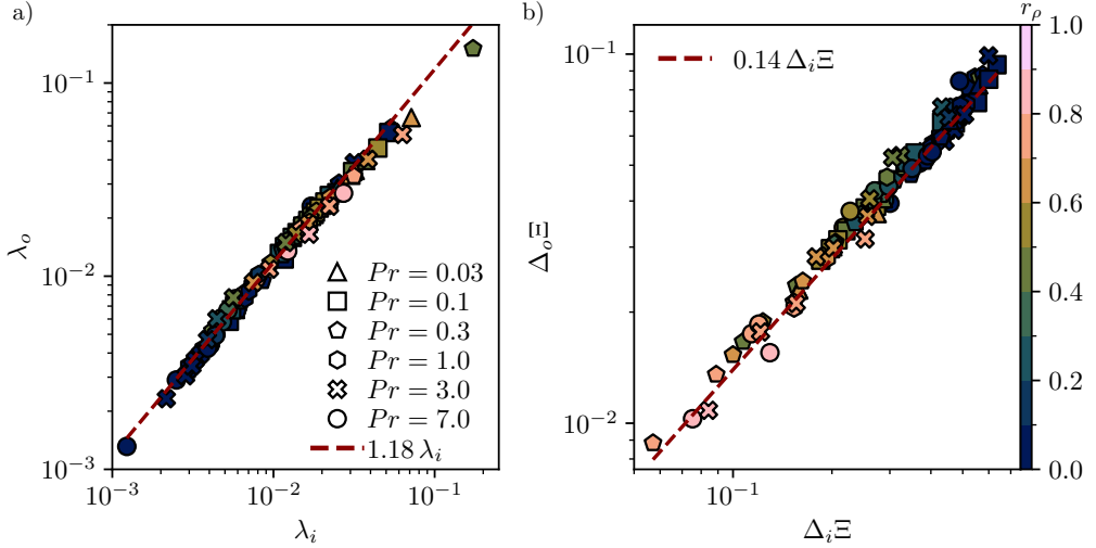
Figure 5: (a) Thickness of the outer boundary layer, \lambda_o , as a function of the thickness of the inner boundary layer, \lambda_i . (b) Composition contrast across the outer boundary layer, \Delta_o \Xi , as a function of its inner counterpart, \Delta_i \Xi . In both panels, the dashed lines correspond to a linear fit to data retaining only those simulations with \lambda_i < 0.02 .
