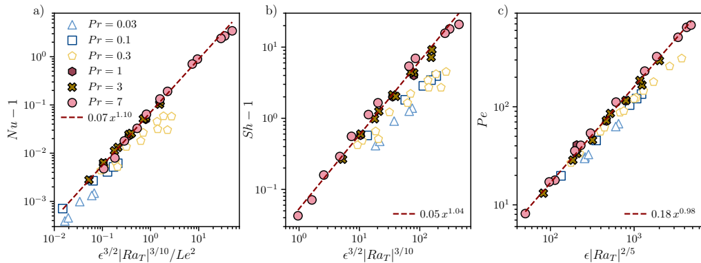
Figure 10: (a) Vertical convective transport Nu - 1 as a function of the theoretical weakly-nonlinear scaling (3.30) for all the simulations with \epsilon < 1 . (b) Vertical convective transport of composition as a function of the scaling (3.31). (c) Convective velocity as a function of the scaling (3.32). The dashed lines correspond to the best fits obtained for the numerical simulations with Pr \geq 1 and \epsilon < 0.5 .
