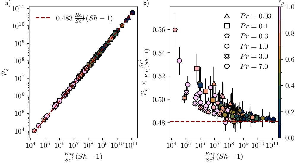
Figure 20: (a) \mathcal{P}_\xi as a function of Ra_\xi Sc^{-2}(Sh-1) . The dashed line corresponds to a linear fit to the data. (b) Compensated scaling of \mathcal{P}_\xi Ra_\xi^{-1} Sc^2 (Sh-1)^{-1} as a function of Ra_\xi Sc^{-2}(Sh-1) . The horizontal line corresponds to the theoretical value derived in Eq. (B 2) for spherical shells with r_i/r_o = 0.35 .
