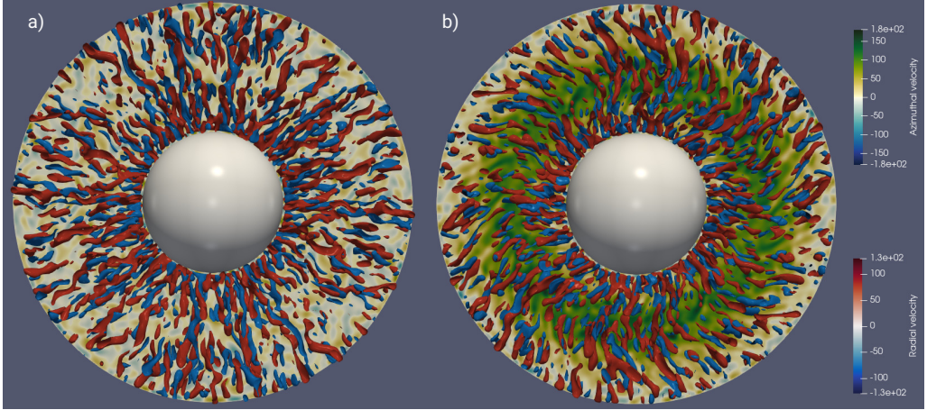
Figure 17: Renderings of the velocity for a numerical model with Pr = 0.3 , Le = 10 , Ra_\xi = 2 \times 10^8 and R_\rho = 5 (simulation 55 in Tab. 3) at t = 3.98 (a) and at t = 5.68 (b). The equatorial plane shows the azimuthal component of the velocity u_\phi , while the red and blue surfaces correspond to the iso-levels of the radial velocity u_r = \pm 80 in the vicinity of the equatorial plane.
