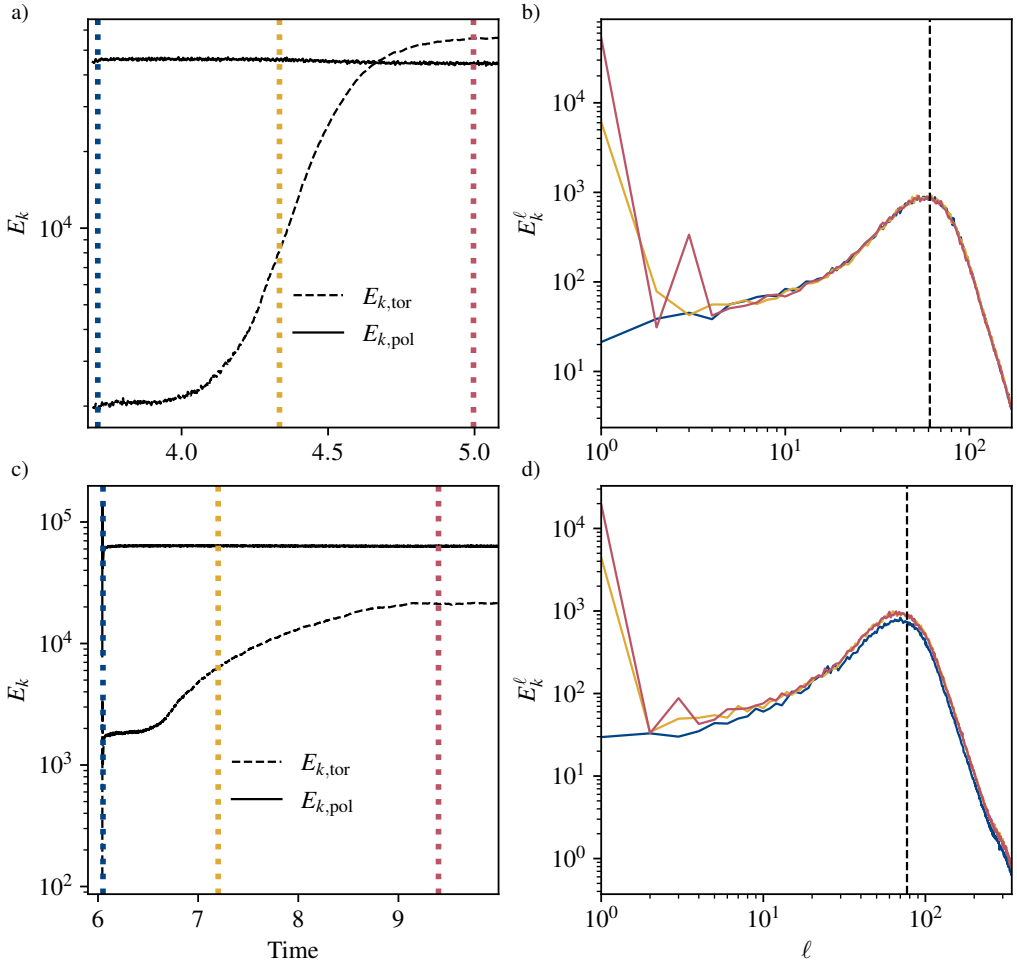
Figure 13: Left panels: time evolution of the poloidal (toroidal) kinetic energy E_{k,pol} ( E_{k,tor} ). Right panels: kinetic energy spectra as a function of the spherical harmonic degree \ell shown at three distinct times which correspond to the vertical dotted lines in the left panels. Panels (a) and (b) correspond to a simulation with Ra_T = -10^8 , Pr = 0.3 , Le = 10 , and R_\rho = 4 (simulation 53 in Tab. 3), while panels (c) and (d) correspond to a simulation with Ra_T = -1.5 \times 10^8 , Pr = 1 , Le = 10 , and R_\rho = 1.3 (simulation 72). In panels (b) and (d), the vertical lines correspond to \ell_h .
