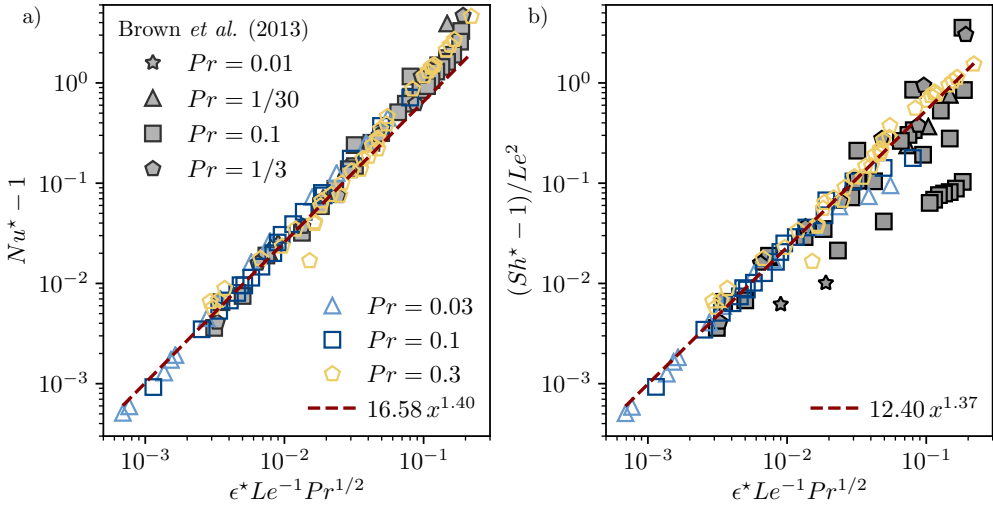
Figure 21: (a) Convective heat transport Nu^* - 1 as a function of \epsilon^* Le^{-1} Pr^{1/2} for our simulations with Pr < 1 alongside the unbounded Cartesian simulations from Brown et al. (2013). (b) Convective transport of chemical composition (Sh^* - 1)/Le^2 as a function of \epsilon^* Le^{-1} Pr^{1/2} . The dashed lines correspond to best fits for the simulations with \epsilon^*/Le < 0.05 . Data from Brown et al. (2013) come from their Table 1.
