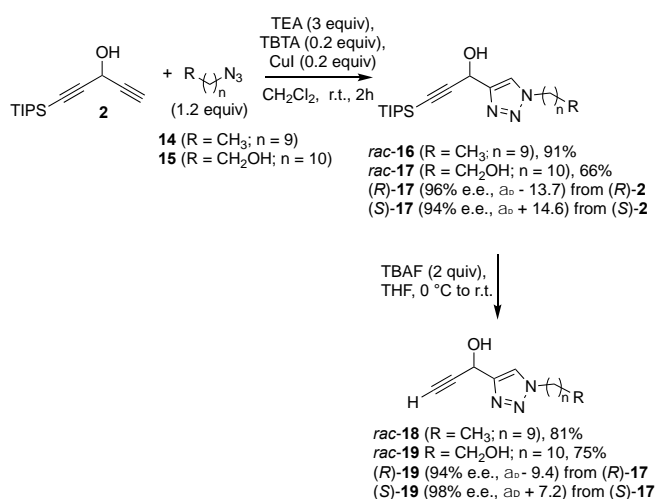
Scheme 4. Derivatization of rac -, (R)- and (S)- 2 via a copper-catalyzed 1,3-cycloaddition reaction to give 1,2,3-triazoles.
