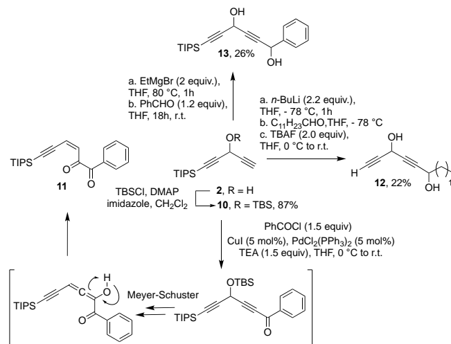
Scheme 3. Selected attempts to react the terminal alkyne of 2 with carbonyl compounds.
