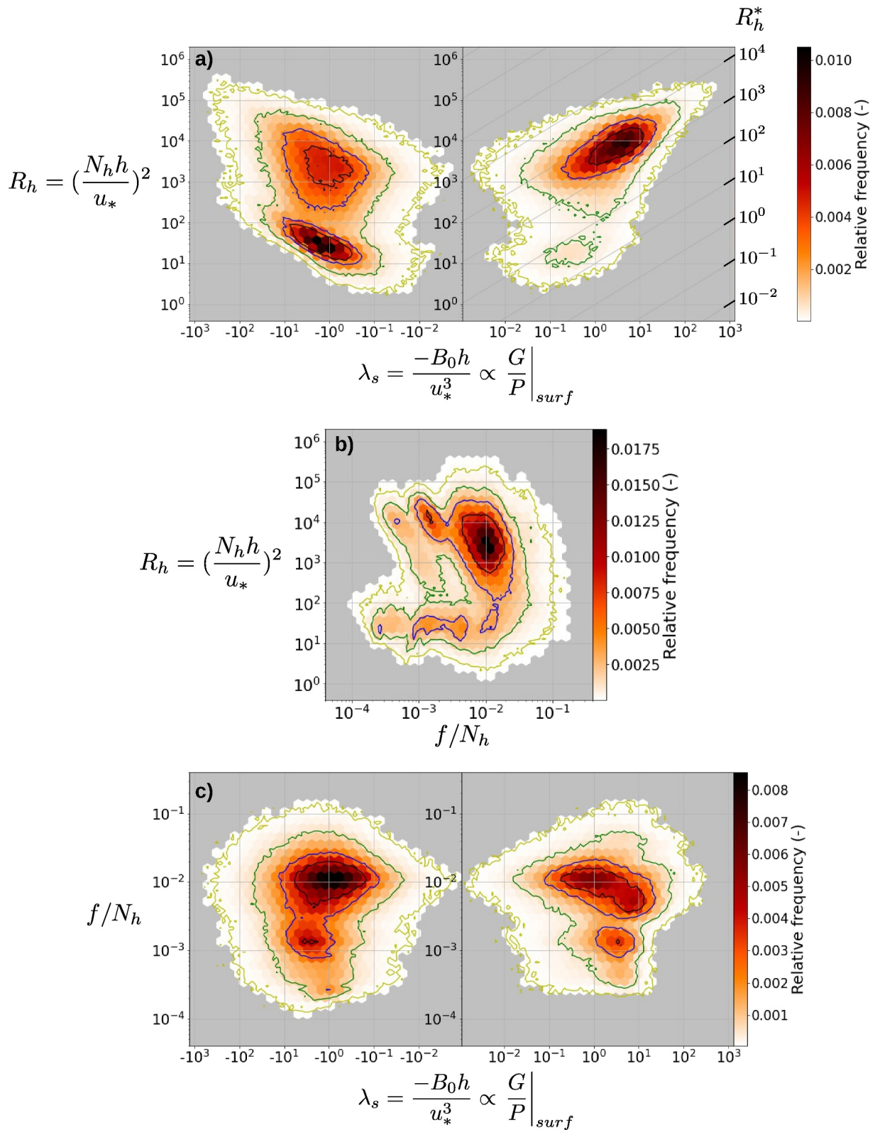
Figure B1. Density maps of the 1D simulations at the global scale for the (a) \lambda_s - R_h^* , (b) f/N_h - R_h and (c) \lambda_s - f/N_h parameter space. The contours of the associated joint Probability Density Functions (PDF) are superimposed. These contours enclose 30 % (black), 60 % (blue), 90 % (green), and 99 % (yellow) of all instances centered at the highest PDF.
