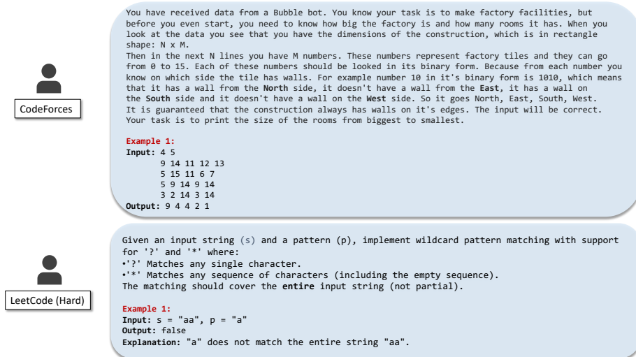
Figure 4. Examples of competitive coding problems from Codeforces and LeetCode.
