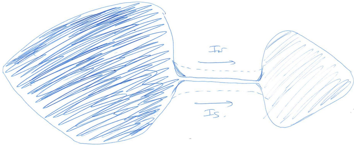
Fig.1: Entropy transport between two reservoirs of superfluid Fermi gases. The system is composed of two reservoirs, connected by a narrow channel. The geometry of the channel can be adjusted from 1D (solid lines) to 2D (dashed lines). A particle and/or entropy imbalance between the two reservoirs leads to particle (resp. entropy) current I_N (resp. I_S ).
