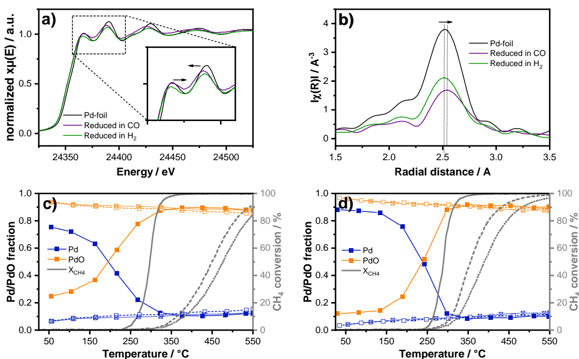
Fig. 5: XANES (a) and Fourier transformed k^3 -weighted EXAFS spectra (b) collected at Pd K edge for the 2 wt.% Pd/ \text{CeO}_2 -120 after reduction by \text{H}_2 and CO. Results of linear combination fitting of the XANES region (-20 eV to 30 eV around the edge) during 3 consecutive light-off/light-out cycles (only light-off curves are depicted) of \text{CH}_4 oxidation following catalyst activation by \text{H}_2 reduction (c) and CO reduction (d). The corresponding methane conversion measured during the operando XAS experiment is plotted as well.
