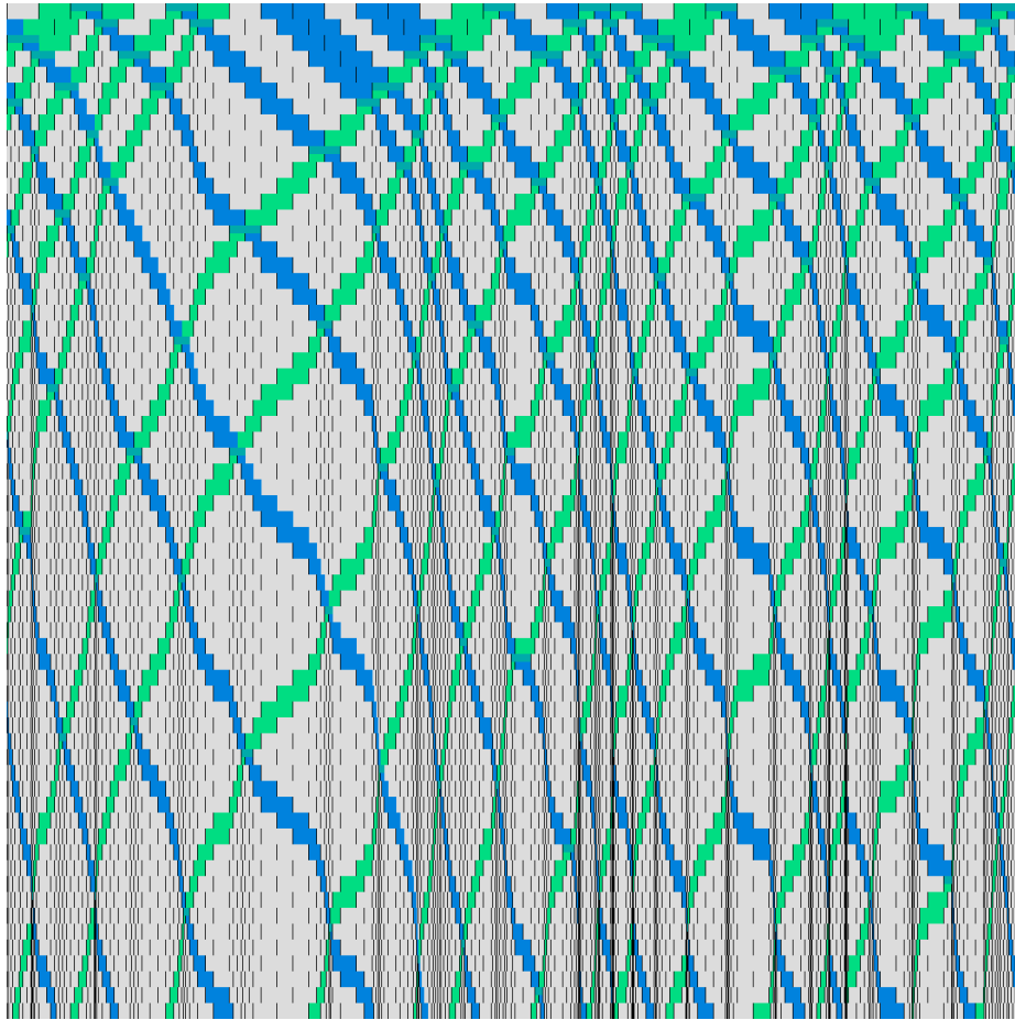
Fig. 3: Spacetime diagram of dynamics \sqrt{7}I . Dynamical clock time flows towards the bottom. Particles corresponding moving along port a (resp. b ) are represented green (resp. blue). Observe how space keeps on expanding, making this spacetime diagram look like a curtain.
