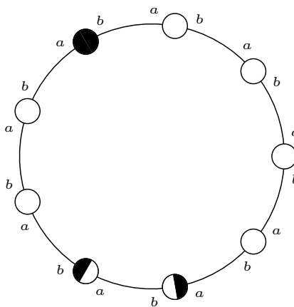
Fig. 1: A configuration. Each full half-disk represents the presence of an (undistinguishable) particle that is about to hop along the corresponding port.
