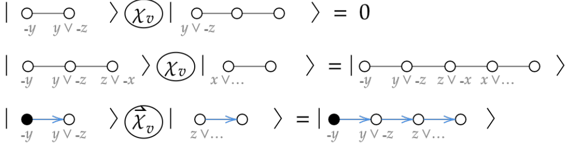
FIG. 5. Generalized tensor product. Here, \chi_v := \zeta_v^1 and \bar{\chi}_v := \bar{\zeta}_v^1 . Top: the two graphs do not correspond to a disk around v and its complement, this goes to zero. Middle: the two graphs correspond to a disk and its complement. Moreover, an edge between them can be derived from names. Below: Same with oriented edges.
