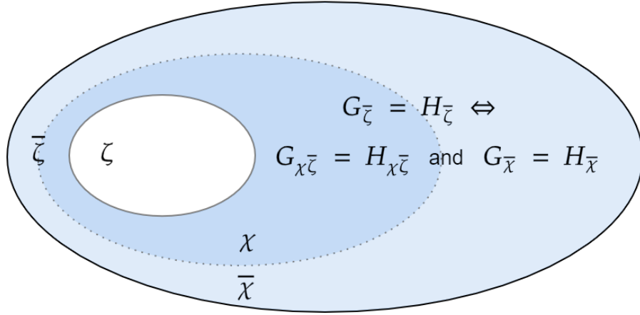
FIG. 3. Comprehension of restrictions \zeta \sqsubseteq \chi demands condition Eq. (2), which states that for any G, H , equality outside the small restriction \zeta (i.e. whether G_{\bar{\zeta}} = H_{\bar{\zeta}} ) may be decomposed as both equality outside \zeta but inside \chi (i.e. whether G_{\chi\bar{\zeta}} = H_{\chi\bar{\zeta}} ), and equality outside \chi (i.e. whether G_{\bar{\chi}} = H_{\bar{\chi}} ). Condition Eq. (2) may fail if a difference lying within \zeta influences the way \chi partitions the outside of \zeta . The condition holds in most relevant cases as shown by Prop. 2. It is needed to establish Lem. 8.
