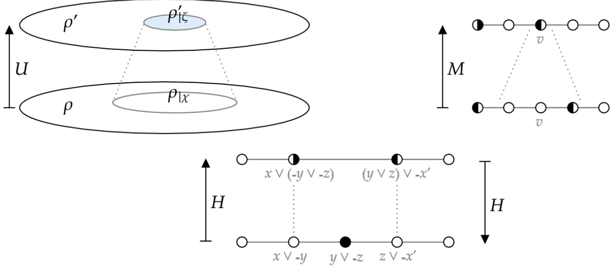
FIG. 9. Causal operators . Left: U \chi\zeta -causal may modify the whole of \rho . But it is such that \rho'_{|\zeta} solely depends on \rho_{|\chi} . Right: \chi_v\zeta_v -causal operator M propagates particles. They bounce on borders. Middle: Causal H is involutive merges/splits all occurrences of these particular patterns, synchronously.
