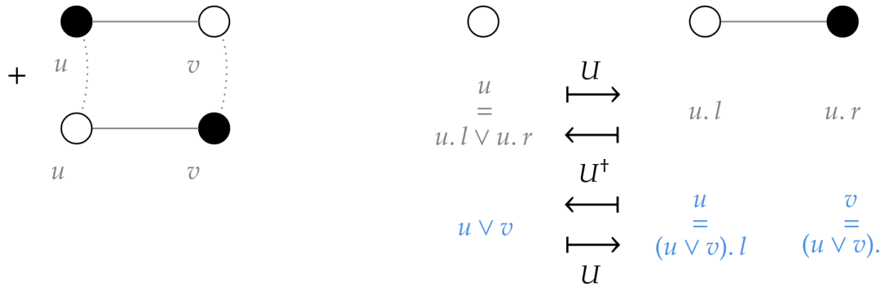
FIG. 1. Necessity of the name algebra. Left: naming vertices is necessary in order to track alignment across quantum superpositions. Right/grey: A quantum evolution may split u into u.l and u.r . As the inverse evolution merges them back we need (u.l \vee u.r) = u . Right/blue: The inverse quantum evolution may also merge vertices u and v into (u \vee v) . As the forward evolution splits them back we need (u \vee v).l = u and (u \vee v).r = v .
