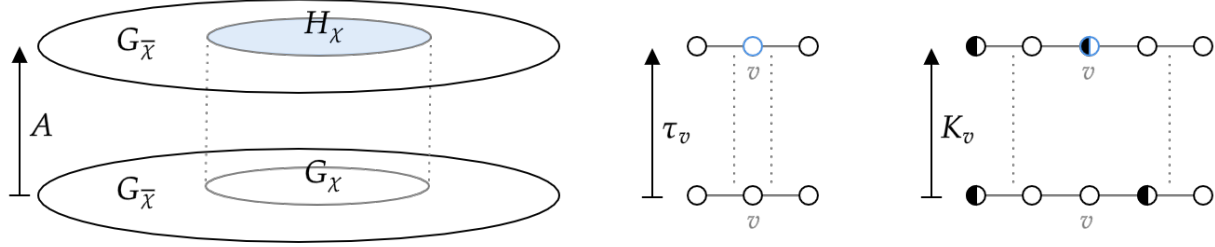
FIG. 7. Local operators. Left: A \chi -local will only modify G_\chi . Middle: \zeta_v -local operator \tau_v just toggles a 'black/blue' bit inside the system at v . Right: \chi_v -local operator K_v is a reversible update rule which computes the future state of the system at v (according to M , see Fig. 9) and toggles it out, whilst attempting to leave the rest mostly unchanged, cf. Th. 1.
