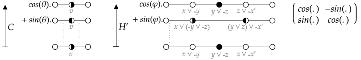
FIG. 10. Causal operators yielding superpositions of states. Left: Instead of simply iterating M , we could iterate MC , where C acts on every right-moving (resp. left-moving) particle by placing it in a superposition of being right-moving with amplitude \cos(\theta) and left-moving with amplitude \sin(\theta) (resp. left-moving with amplitude \cos(\theta) and right-moving with amplitude -\sin(\theta) ). Right: Instead of simply merging or splitting according to H , we could do so in a superposition. Here the splitting applies with amplitude \sin(\varphi) . Similarly the merge needs be applied with amplitude -\sin(\varphi) . Lastly, we may compose these, e.g. U = H'MC makes for an interesting quantum causal graph dynamics.
