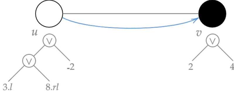
FIG. 2. Graphs. Left: A system with state 'white' and name u = ((3.l \vee 8.rl) \vee -2) . Right: A system with state 'black' and name v = (2 \vee 4) . Middle/grey: Here we decided to interpret u.r = -2 and v.l = 2 as the presence of an unoriented edge \{u, v\} . Middle/blue: We could have chosen to interpret it as an oriented edge (u, v) instead. Middle: In both cases, geometry is derived from relative information that is already present within systems, and which is invariant under renamings.
