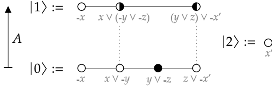
FIG. 8. Strict locality. 1/ Local but not strictly. Let \chi := \zeta_x^2 . Consider A = |1\rangle\langle 0| . It is \chi -local because \langle H|A|G\rangle \neq 0 if and only if |G\rangle = |G_\chi\rangle = |0\rangle and |H\rangle = |H_\chi\rangle = |1\rangle . It is not strictly \chi -local because \langle 02|A^\dagger A|02\rangle = 0 \neq 1 = \langle 0|A^\dagger A|0\rangle\langle 2|2\rangle . It is not \chi -consistent-preserving because |0\rangle \otimes |2\rangle \neq 0 yet |1\rangle \otimes |2\rangle = 0 . 2/ Strictly local. Let \xi be the restriction that selects |0\rangle or |1\rangle whatever their context, and returns the empty graph if they do not occur. Then U := (|0\rangle\langle 1| + |1\rangle\langle 0| + |\emptyset\rangle\langle \emptyset|) \otimes I is unitary, strictly \xi -local and \xi -consistent preserving.
