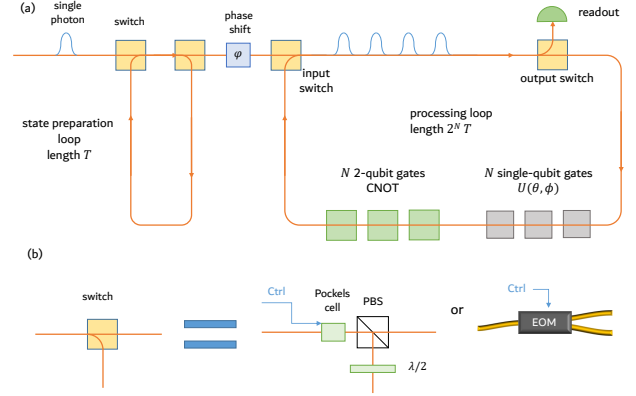
FIG. 2. (a) Scheme of the qudit processor architecture. (b) Possible implementation of the photonic switches. The proposed implementations of single- and two-qubit gates (resp. gray and green squares) are detailed in figures 5 and 7.
