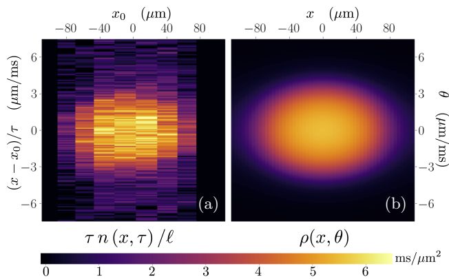
Figure 2. (a) Rescaled density profiles \tau n/\ell with \tau = 40 ms and \ell = 37\mu\text{m} for the different slices of Fig. 1(c), centered on different positions x_0 . (b) Theory prediction for the rapidity distribution \rho(x, \theta) at thermal equilibrium in the potential V(x) at the temperature T_{\text{YY}} and chemical potential \mu_{\text{YY}} (obtained by fitting the in situ profile in Fig. 1(d)).
