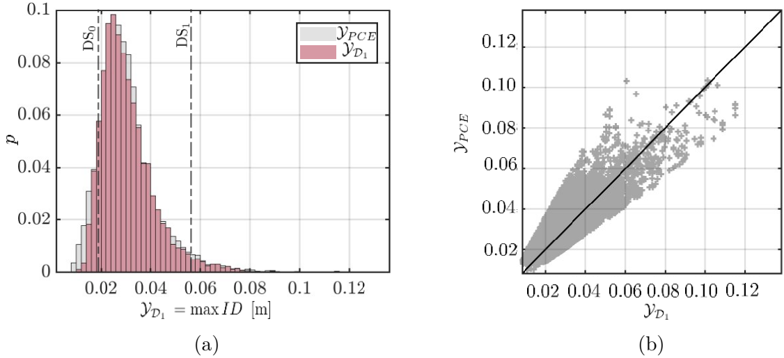
Figure 13: (a) Comparison of the histograms for the outputs, \mathcal{Y}_{PCE} , of the PCE metamodel and the EDPs, \mathcal{Y}_{D_1} , of the \mathcal{D}_1 dataset, i.e., the initial damage state condition DS_1 , and (b) the associated validation \mathcal{Y}_{D_1} - \mathcal{Y}_{PCE} plot.
