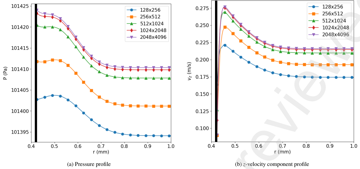
Fig. 18. Pressure and z -velocity component profiles along r -axis at z = z_1 and t = t_1 for five different grids
