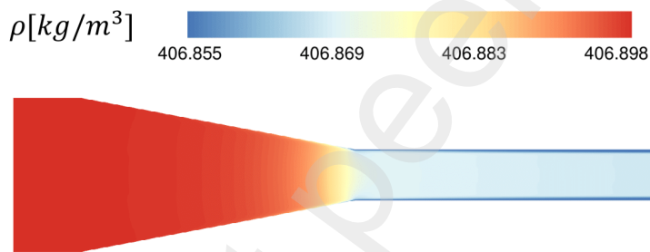
Fig. 11. Density field in the convergent pipe.
