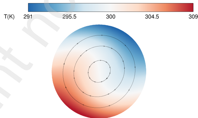
Fig. 8. Temperature field and streamlines at steady state for the Rayleigh numbers Ra = 23000 with an imposed local heat flux (INBC) for the grid 256 \times 256 .
