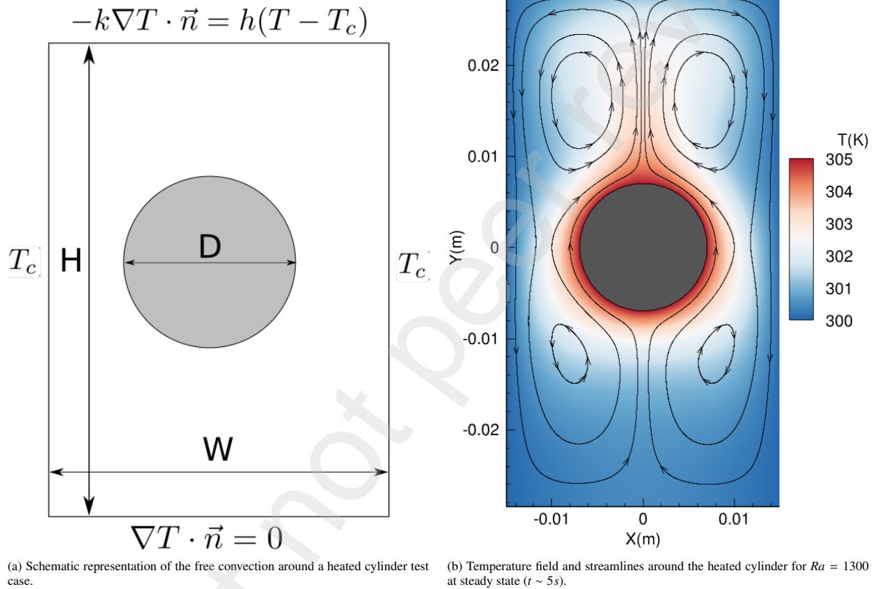
Fig. 5. Configuration (a) and temperature field snapshot (b).
