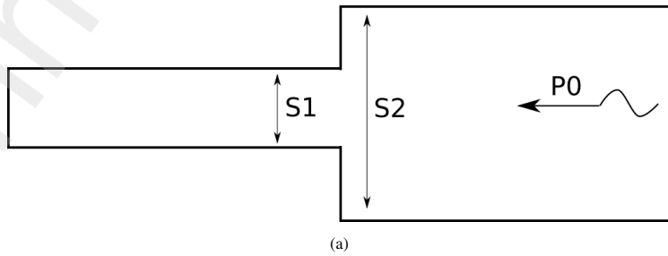
Fig. 13. Schematic representation of the test case with 2 surfaces S_1 and S_2 and the pressure wave on the right with a pressure drop p_0 = p_{atm} - p
