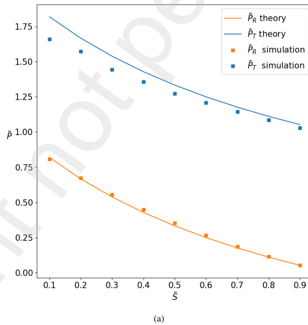
Fig. 16. Comparison between numerical simulations and theory on the variations of \tilde{p}'_R and \tilde{p}'_T with \tilde{S} for the grid 512 \times 3072 . The blue curve is the transmitted pressure and the orange curve is the reflected pressure ratio.
