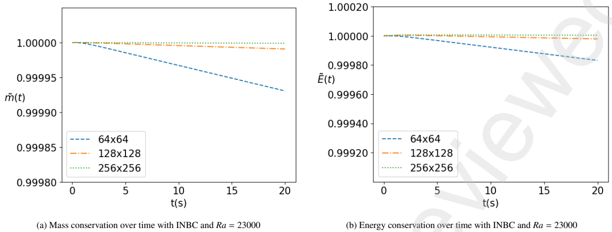
Fig. 9. Temporal evolution of the total energy and mass for different grids 64x64, 128x128, 256x256 with Ra = 23000 for INBC.
