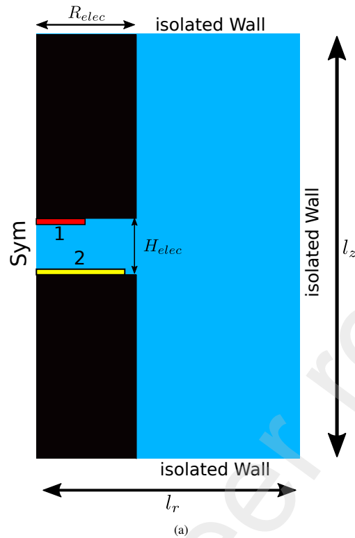
Fig. 21. Schematic representation of the axisymmetric domain. The outer walls are isolated thermally and electrically. The imposed electric flux is represented on the zone 1. The constant electric potential which absorb the current is the zone 2. All the other surfaces are isolated electrically.
