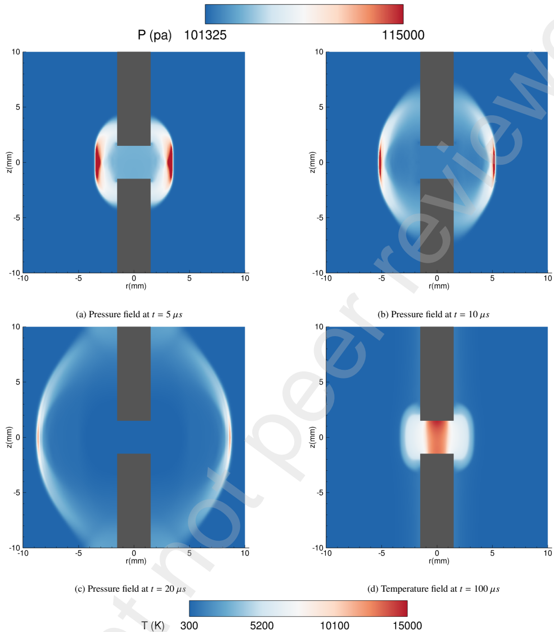
Fig. 23. Acoustic wave on 23a, 23b and 23c. The Temperature field on 23d
