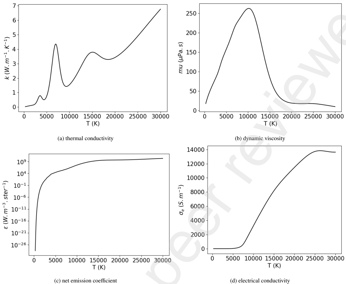
Fig. B.25. The graphs of transport properties of air.
