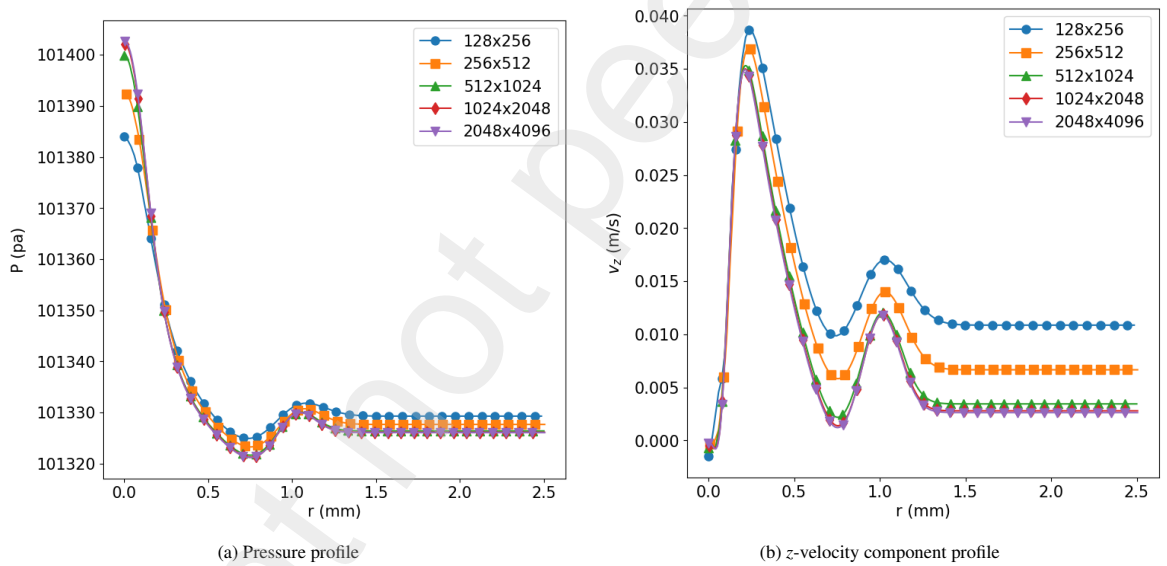
Fig. 19. Pressure and z -velocity component profiles along r -axis at z = z_1 and t = t_1 for five different grids
