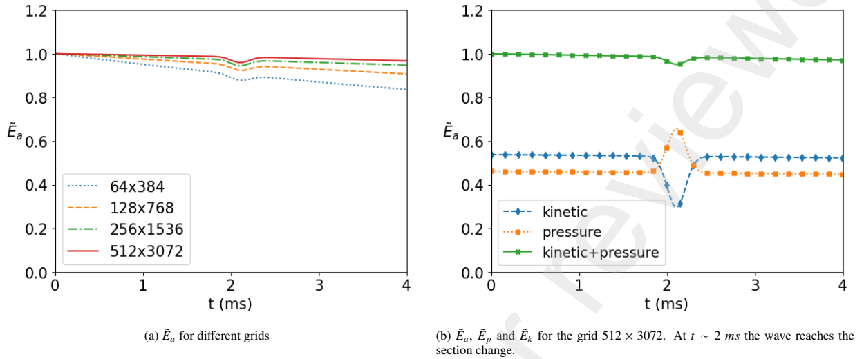
Fig. 15. Temporal evolution of dimensionless energies \tilde{E}_a
