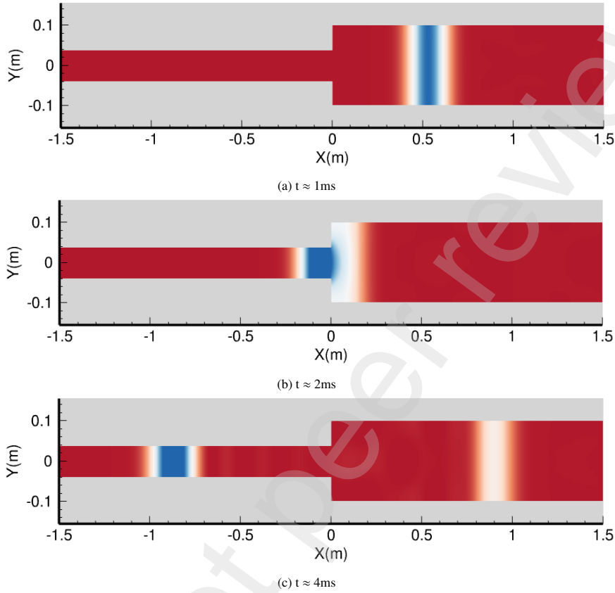
Fig. 14. Pressure profile in the tube at different times for the grid 512 \times 3072
