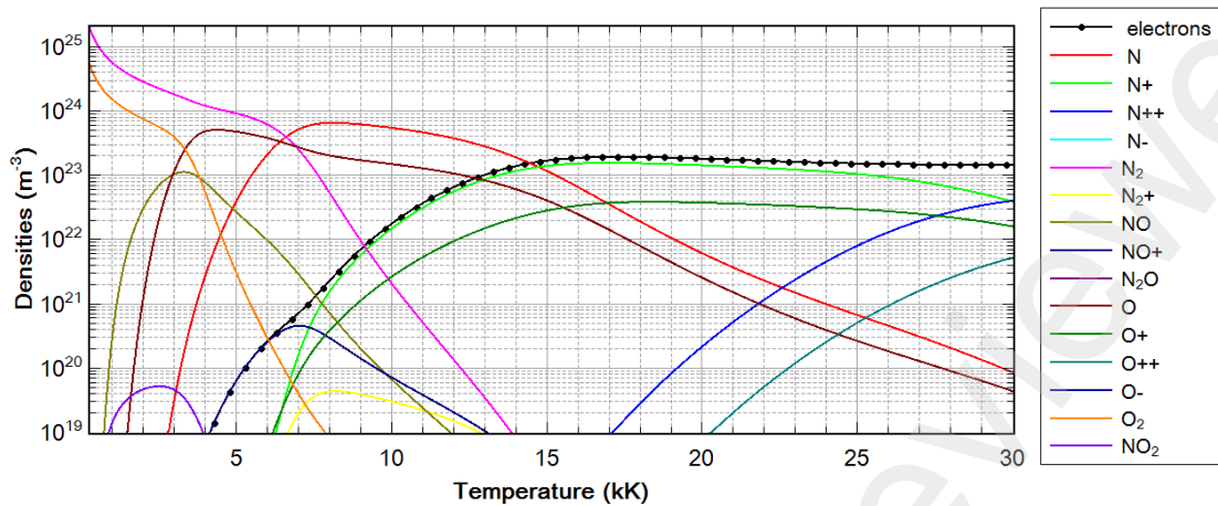
Fig. 1. L.T.E. composition of an air thermal plasma at atmospheric pressure
