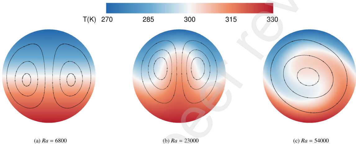
Fig. 7. Temperature field and streamlines at steady state for the three different Rayleigh numbers with an imposed temperature (IDBC) for the grid 256 \times 256 .
