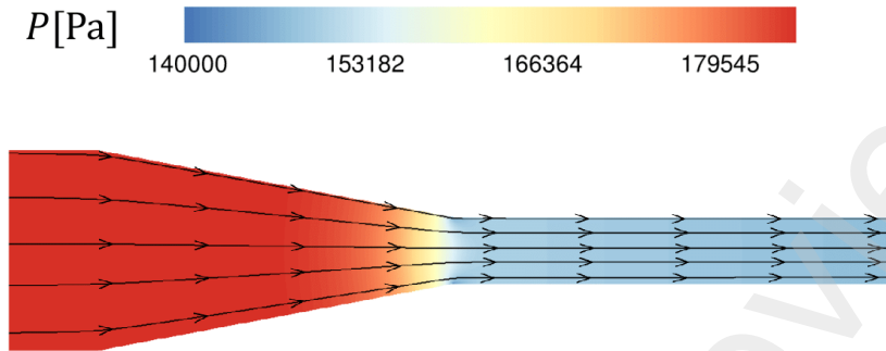
Fig. 10. Pressure field and streamlines in the convergent pipe.
