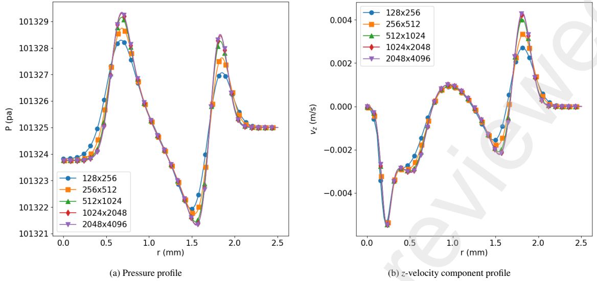
Fig. 20. Pressure and z -velocity component profiles along r -axis at z = z_1 and t = t_1 for five different grids
