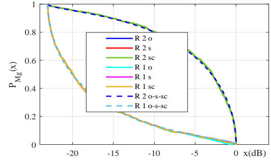
Fig. 10. P_{M_g}(x) as a function of x ( N = 1 , M = 1, 2 , \epsilon_s = 10 dB, \epsilon_1 = 20 dB, \omega = 0 , deterministic channels, R signals.
