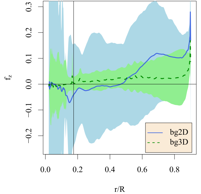
Fig. 9. Radial profile of the time-averaged filling factor f_z as defined in Eq. (14) for 2D and 3D simulations of the 3M_{\odot} red giant star. The shaded regions represent one standard deviation above and below each time-averaged line. The radial position of the convective boundary determined by the Schwarzschild criterion is indicated by a vertical black line.
