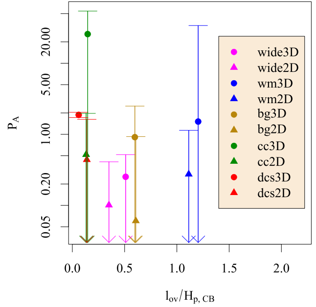
Fig. 11. Anders penetration parameter P_A vs the overshooting depth in units of the pressure scale height at the convective boundary determined by the Schwarzschild criterion l_{\text{ov}}/H_{p,\text{CB}} for all 2D and 3D simulations described in Table 1. Error bars consider one standard deviation of the convective flux at each of the two radial points that contribute to this number. A logarithmic scale is applied to the vertical axis because this parameter, as formulated, can be larger than one.
