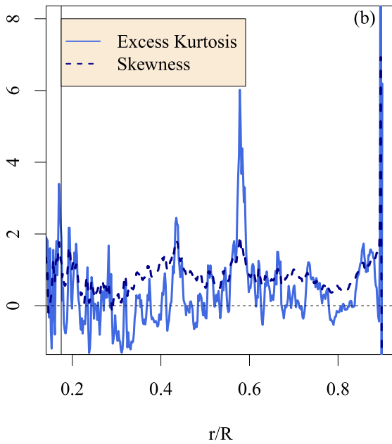
Fig. 13. Time-averaged profiles of skewness and excess kurtosis of the width of inflows for the red giant simulations (a) in bg2D, and (b) bg3D. The radial position of the convective boundary determined by the Schwarzschild criterion is indicated by a vertical black line.
