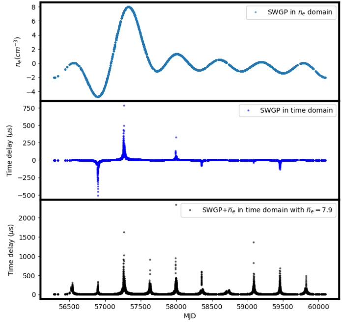
Fig. 1. Sample results from one SWGP realization. In a hypothetical scenario, considering the long time span of one of the pulsars in our dataset PSR J1022+1001. The top panel shows the variations in n_e that can be modelled using SWGP perturbed from the mean value. The middle panel shows the corresponding time delays due to SWGP. The bottom panel shows the time delay when the deterministic signal with an \bar{n}_e of 7.9 is added on top of SWGP.
