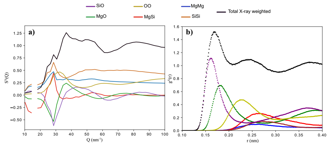
Fig. 3 | AIMD calculations on \text{MgSiO}_3 glass Hugoniot at 6000 K ( P = 167 GPa; density of 5.17 \text{ g/cm}^3 ). a Total and partial X-ray weighted (see Methods and Figure S7) structure factors S^X(Q) . b Total and partial X-ray weighted (see Methods and Figure S6) radial distribution functions g^X(r) .
