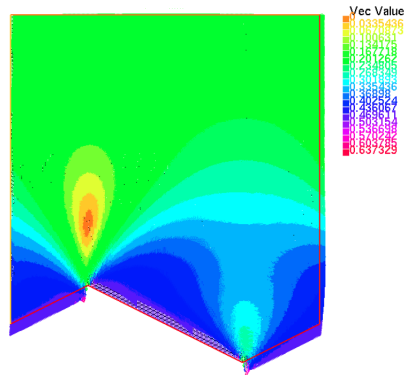
Figure 4.5: Solution with no curvature constraint ( M_2 = +\infty ) and J \approx 0.196
