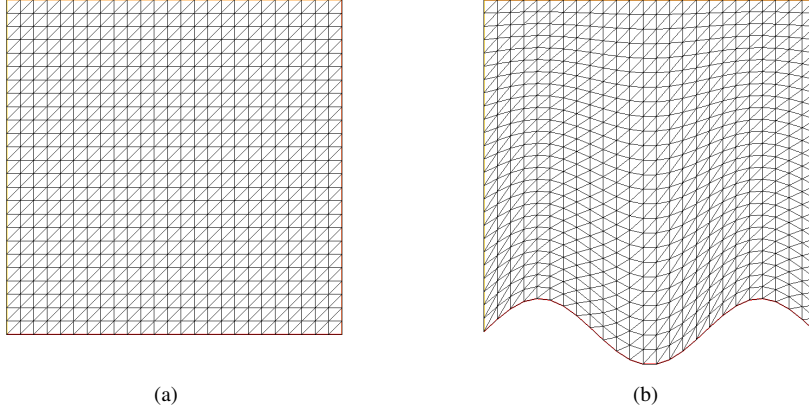
Figure 4.2: Fluid domain mesh: (a) initial; (b) modified for f(x) = 0.1 \sin(3\pi x) .
