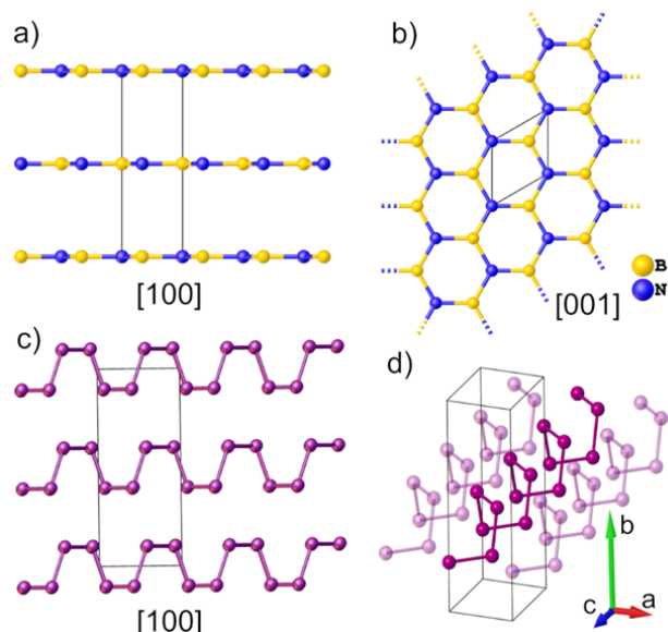
Fig. 1 Crystalline structures of hBN (a,b) and bP (c,d). hBN exhibits a planar conformation of the layers (a), while bP forms puckered layers (c). Panel b and d highlight the intra-layer differences between a planar layer of hBN (b) and the armchair conformation of a layer of bP.
