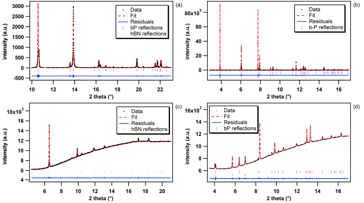
Fig. 2 Integrated XRD patterns of hBN (panel a,c) and bP (panel b,d) in run 1 to 3 and their corresponding Le Bail fittings. (a) Run 1 (Ambient pressure, T=300 K; the XRD patterns were collected simultaneously), (b) Run 2 (Ambient pressure, T=300 K), (c) and (d) Run 3 (Ambient pressure, T=300 K). The higher background in run 2 and 3 is due to the small sample dimension and high X-ray Compton scattering signal from the diamond anvil cell.
