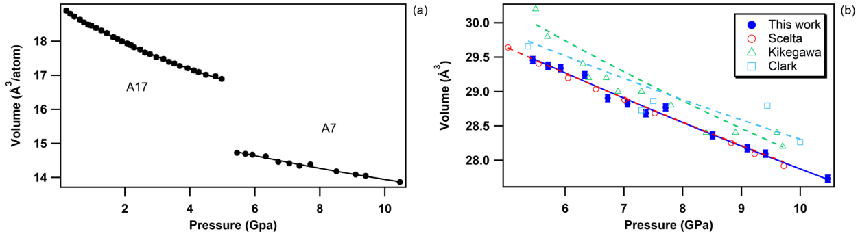
Fig. 8 (left) Equation of state of bP at room temperature across the orthorhombic to rhombohedral (A7) first-order phase transition, observed at 5 GPa. (right) Unit-cell volume evolution of A7 rhombohedral P in the 5 – 10.5 GPa pressure range at room temperature. The solid blue circles represent the data acquired in the present study. The empty symbols refer to the data reported by Scelta et al. [43] (red circles), Kikegawa et al. [44] (green up triangles) and Clark et al. [81] (blue squares). The corresponding EoS fits are represented by lines.
