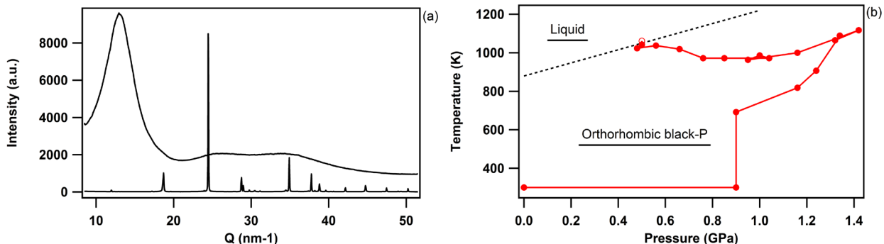
Fig. 10 Determination of a melting point of bP using the anisotropic thermo-elastic properties of bP. (Left) Melting criteria: At the melting the Bragg reflections of bP disappear (bottom XRD pattern) and a liquid diffuse signal appears (upper XRD pattern). (Right) P, T pathway of the XRD data collection. Solid red circles indicate crystalline bP, while the empty red circle indicate the liquid state. The dotted line represents the melting line of bP.
