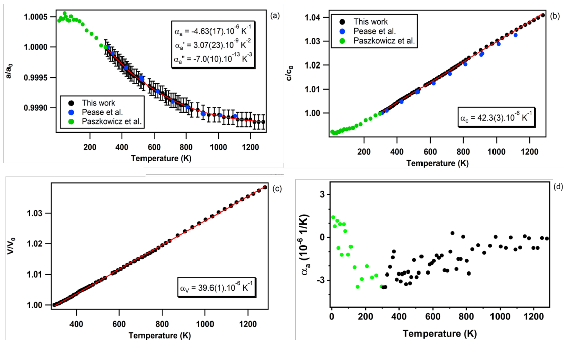
Fig. 3 Relative temperature variation of the a and c lattice parameters of hBN with respect to their room T values at ambient P , respectively along the [100] (panel a) and, [001] (panel b) directions. The relative volumetric thermal expansion and temperature evolution of the linear thermal expansion along the a crystallographic axis are displayed in panel c and d, respectively. Symbols correspond to the experimental data from this (black) and literature (blue and green) studies, whereas the red curves are linear or polynomial fits of our data. Error bars in the last three panels are smaller than the size of the plotted points.
