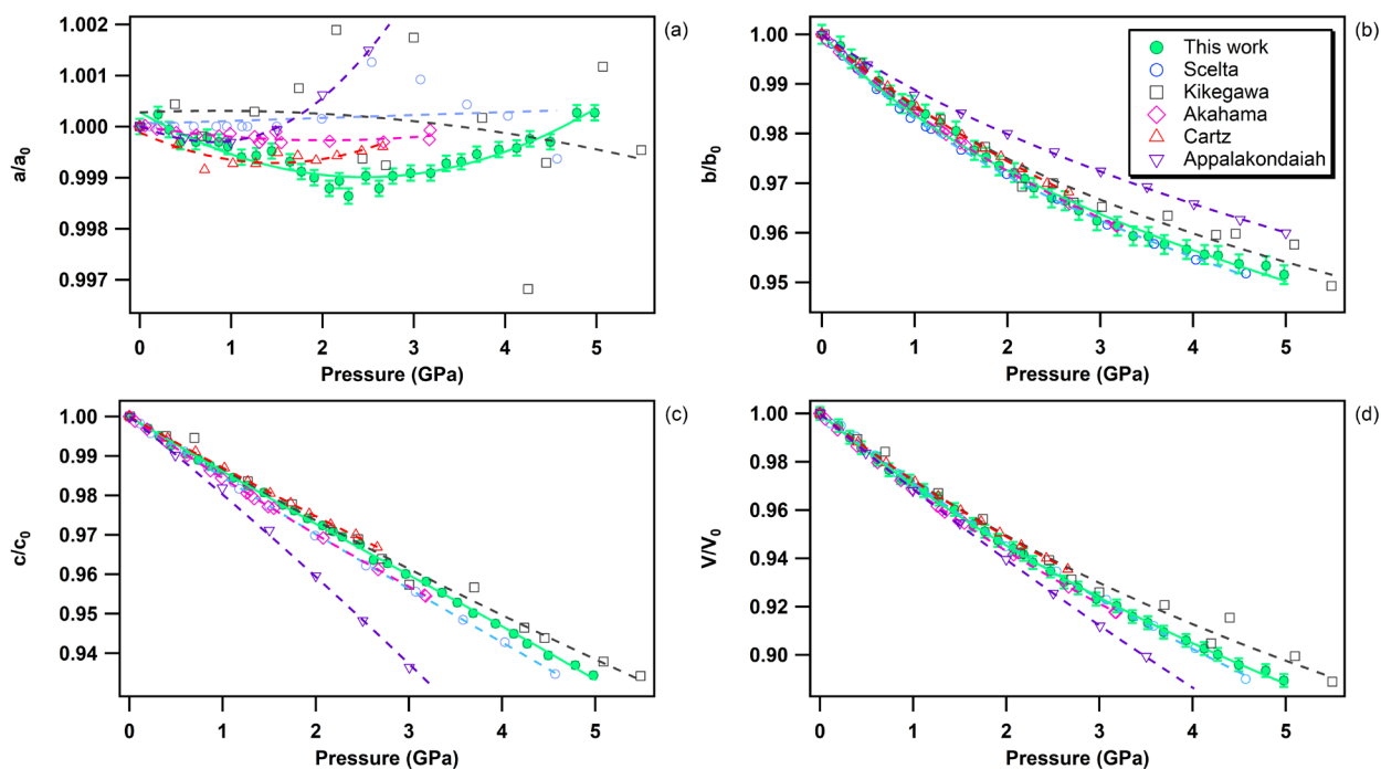
Fig. 7 Relative lattice parameters and unit-cell volume variation of bP in the 0-5 GPa pressure range at room temperature. The solid green circles represent the data obtained in the present study. The empty symbols refer to the data reported in the literature. Blue circles : Scelta et al. [43]; black rectangles; Kikegawa et al. [44]; pink diamonds; Akahama et al. [45]; red up triangles; Cartz et al. [46]; and, violet down triangles; Appalakondaiah et al. [47]. The individual a , b and c -axis data were fitted using a polynomial equation and the volume data using a third order Birch-Murnaghan equation of state [80].
