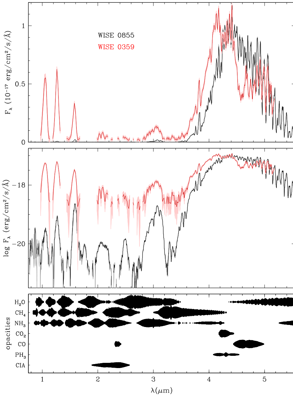
Figure 3. NIRSpect PRISM spectra of WISE 0855 (this work) and the Y0 dwarf WISE 0359 (Beiler et al. 2023) on linear and logarithmic flux scales (top and middle). The spectrum of WISE 0359 has been scaled to roughly match the data for WISE 0855 at 4–5 \mu\text{m} . Uncertainties of \pm 1\sigma are plotted as gray and pink bands. Fluxes that are consistent with zero ( F_\lambda - \sigma \leq 0 ) have been omitted. The bottom panel shows a representation of opacities in which the vertical thickness of each band is proportional to the logarithm of the abundance-weighted absorption cross section for a given molecule at P = 1 bar and T_{\text{eff}} = 250 K (bottom). The opacities of \text{CO}_2 , \text{CO} , and \text{PH}_3 have been scaled by factors of 1000, 100, and 1000, respectively, so that their strongest features are visible.
