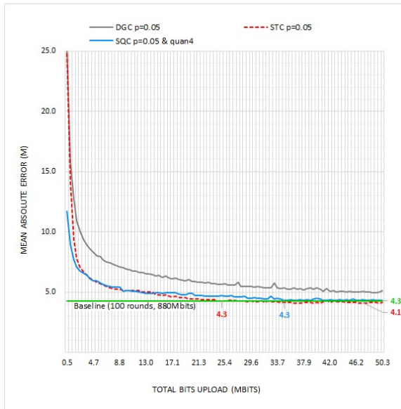
Figure 2. Communication cost vs MAE - SGD Optimizer
