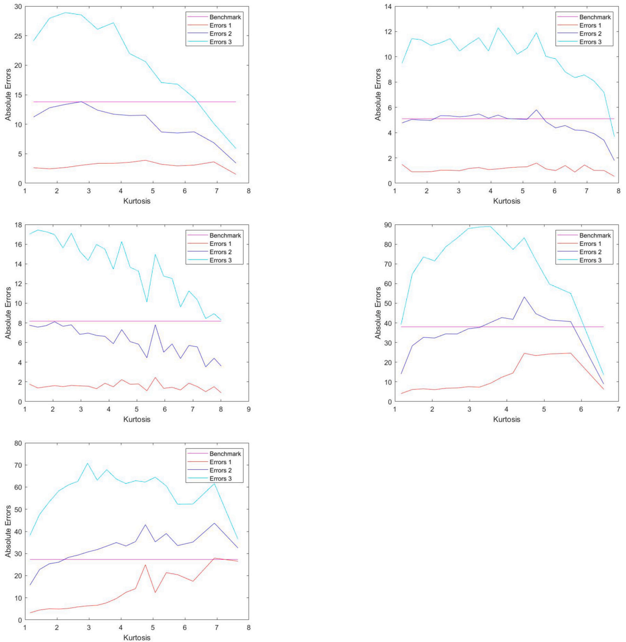
Fig. 4. Prediction errors for the kurtosis including benchmark errors. The five graphs correspond to the five initial weight distributions: (top left) uniform distribution, (top right) Beta distribution with \gamma = 1 and \beta = 3 , (center left) Beta distribution with \gamma = \beta = 0.5 , (center right) Beta distribution with \gamma = \beta = 2 , (bottom left) Beta distribution with \gamma = 1 and \beta = 0.5 .
