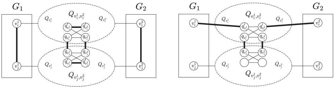
FIGURE 5 On the left, v_i, v_j are covered by the matching-cut of G , and so we take v_i^1v_i^1, v_i^2v_i^2 in the perfect matching-cut of G' . On the right, v_i is not covered by the matching-cut of G , and so we take v_i^1q'_{v_i^1}, v_i^2q'_{v_i^2} in the perfect matching-cut of G' .
