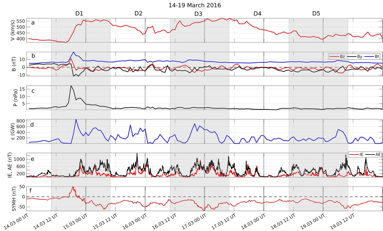
Figure 1. Overview of solar wind and geomagnetic indices for the 14 March 2016 storm. The parameters are as follows: (a) solar wind speed, (b) interplanetary magnetic field magnitude B_r , and B_y and B_z components in the geocentric solar magnetospheric coordinates (GSM), (c) solar wind dynamic pressure, (d) Akasofu \epsilon parameter, (e) AE and IE indices, and (f) SYM-H index. The shaded/unshaded areas represent days in format D1–D5 as described in the text.
