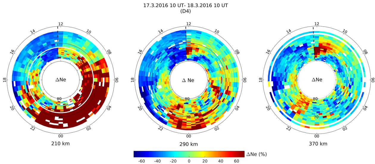
Figure 6. \Delta N_e in percentage for D4 at different heights: 210, 290, and 370 km.
