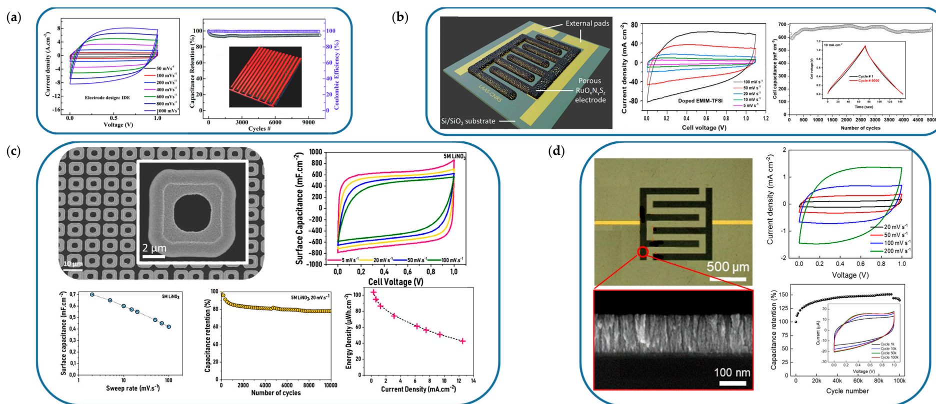
Figure 8. Metal oxide electrode materials for on-chip micro-supercapacitor applications. (a) Sputtered anhydrous \text{RuO}_2 thin-film electrodes. CV measurement, and stability of the interdigitated MSC of 10,000 cycles. Reproduced with permission from [247]. Copyright (2017), John Wiley & Sons-Books. (b) All-solid-state interdigitated microdevice based on porous \text{RuO}_x\text{N}_y\text{S}_z . CV plots in doped PVA and doped [EMIM][TFSI] at different scan rates, and cell capacitance retention with the number of charge/discharge curves at 10 \text{ mA}\cdot\text{cm}^{-2} (inset: 1st and 5000th potential-time curve during GCD). Reproduced with permission from [257]. Copyright © 2024, American Chemical Society. (c) 3D interdigitated MSCs based on electrodeposited \text{MnO}_2 . Top view SEM images of the 3D MSC, CV of a 3D MSC in parallel plate configuration measured in 5 \text{ M LiNO}_3 vs. the sweep rate, evolution of the surface capacitance, capacitance retention, and real energy density of the MSC, respectively. Reproduced with permission from [250]. Copyright (2021), Elsevier. (d) Interdigitated MSCs operating in physiological electrolytes based on sputtered iridium oxide films (SIROFs). SEM images of SIROF in cross-sectional view, CV measurements, and cycle stability of SIROF MSC over 100,000 CV cycles at 200 \text{ mV}\cdot\text{s}^{-1} . Reproduced with permission from [245]. Copyright (2022), IOP Publishing.
