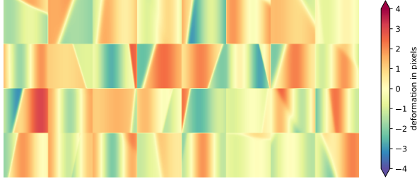
Fig. 27. Examples of simulated flows (x component)
