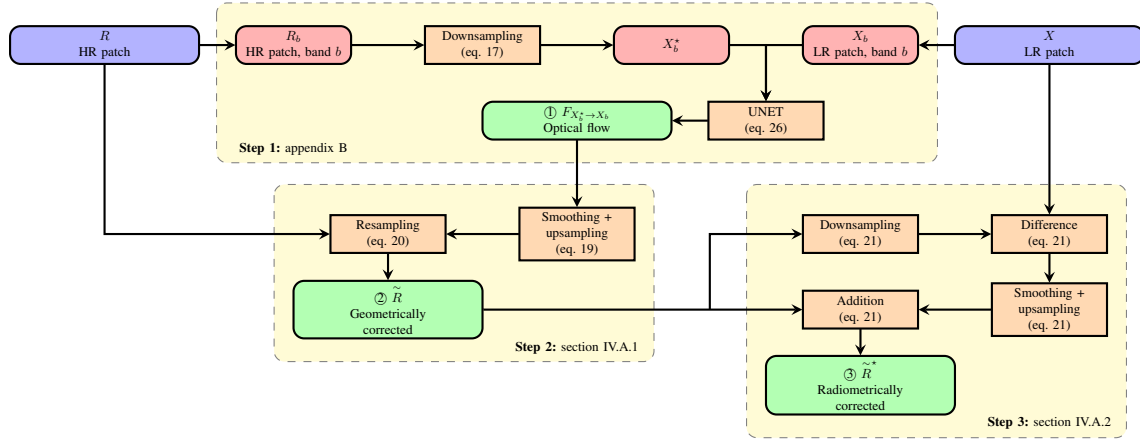
Fig. 12. Overview of robust strategy workflow. Outputs of the three main steps are highlighted in green.
