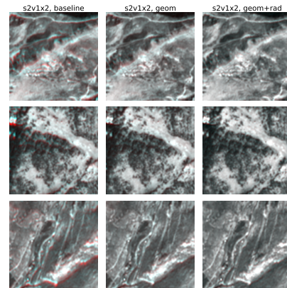
Fig. 18. Color composition highlighting geometric discrepancies for SISR models trained on the s2v1x2 training set with the different strategies (R: B4 from Sentinel-2, B, G: B4 SISR predicted image). Geometric discrepancies appear in red or blue.
