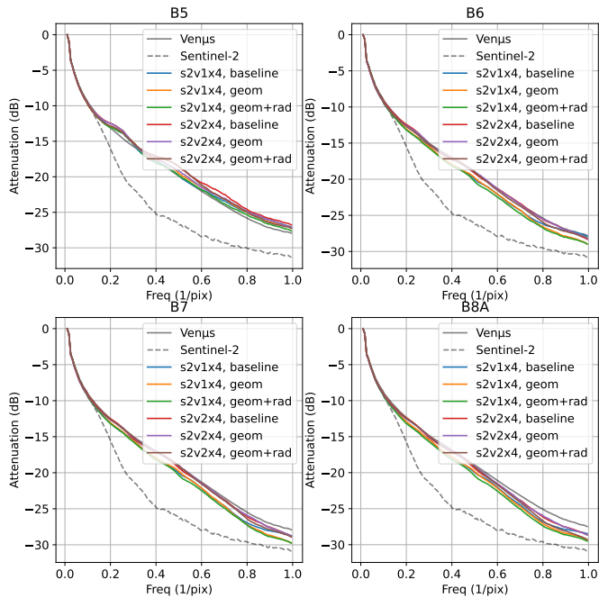
Fig. 32. Frequency Domain Analysis for baseline and proposed robust strategy of the Sen2Venüs, 20 m → 5 m experiment with s2v1x4 and s2v2x4 training sets, evaluated on the Sen2Venüs testing set.
