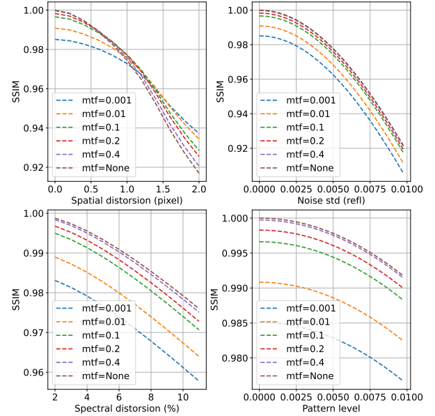
Fig. 5. Benchmarking of SSIM (higher is better) with respect to geometric distortion, radiometric distortion, noise level and chessboard pattern level, for different level of blur, ranging from mtf=None (no blur applied) or mtf=0.4 (very sharp images) to mtf=0.001 (very blurry images)
