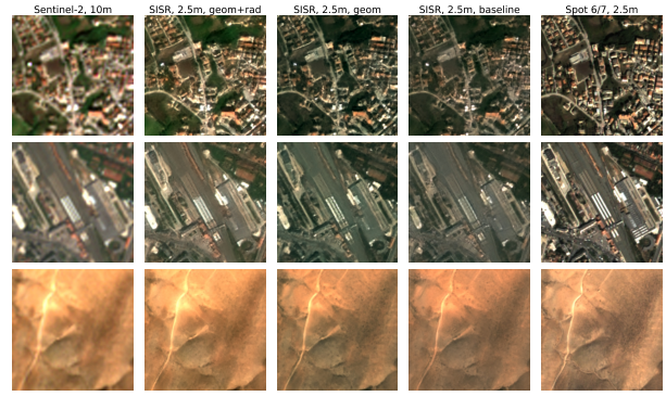
Fig. 16. Examples of predicted patches (Color composition: B4, B3, B2) from the testing set of Worldstrat, for SISR model trained on wsx4 training set, with baseline, geom and geom+rad strategies. Note that the input image Sentinel-2 patches of first column have been up-sampled with bicubic interpolation (a larger version of this figure can be found in the supplementary materials).
