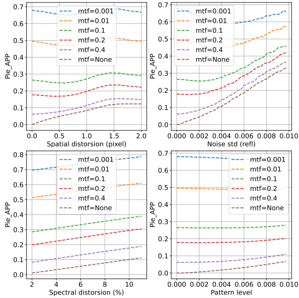
Fig. 24. Benchmarking of PieAPP (lower is better) with respect to geometric distortion, radiometric distortion, noise level and chessboard pattern level, for different level of blur, ranging from mtf=0.4 (very sharp images) to mtf=0.001 (very blurry images)
