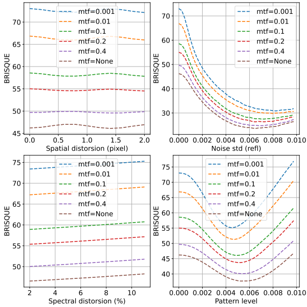
Fig. 7. Benchmarking of BRISQUE (lower is better) with respect to geometric distortion, radiometric distortion, noise level and chessboard pattern level, for different levels of blur, ranging from mtf=0.4 (very sharp images) to mtf=0.001 (very blurry images)
