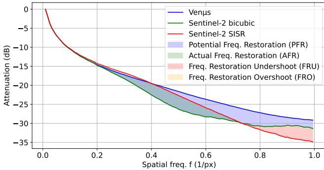
Fig. 9. Illustration of Potential Frequency Restoration (PFR), Actual Frequency Restoration (AFR), Frequency Restoration Overshoot (FRO) and Undershoot (FRU) based on logarithmic normalized Frequency Attenuation Profiles ( \mathcal{F}_{AP}^* ) from Venus patches, bicubic up-sampled Sentinel-2 and a SISR prediction. Spatial frequencies in x axis correspond to normalized spatial frequencies f = \frac{f_n}{f_N} .
