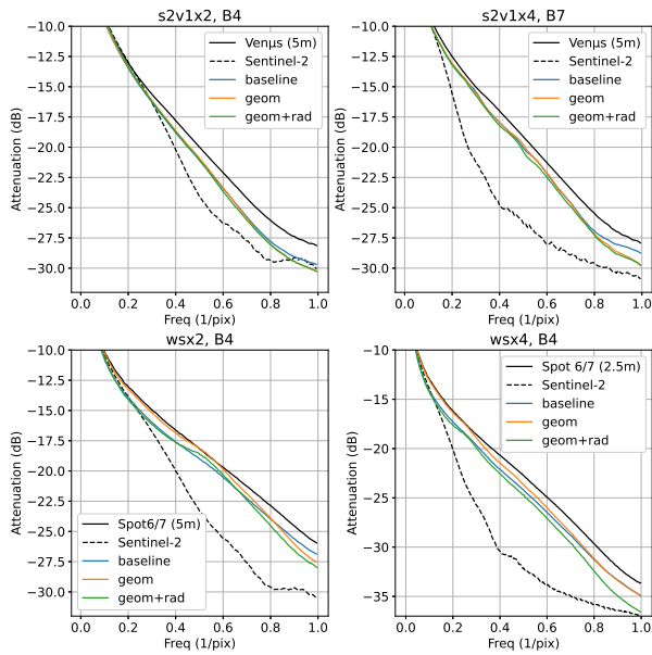
Fig. 13. Impact of proposed strategies on the \mathcal{F}_{AP}^* for each of the training set, for band B4 (except for training set s2v1x4 , where band B7 is used).
