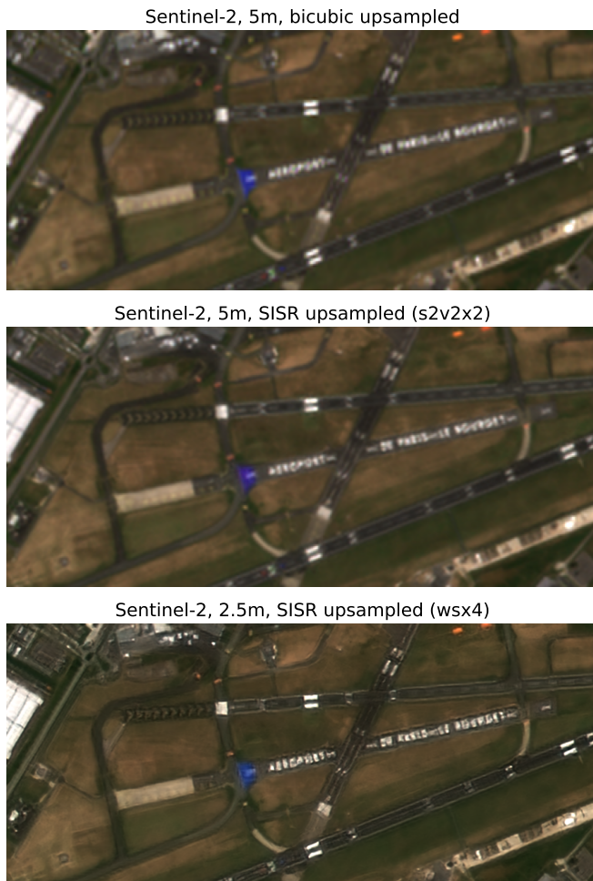
Fig. 22. Can you read it ? Sentinel-2 image of Le Bourget airport, France. From top to bottom, Sentinel-2 up-sampled to 5 m with bicubic, Sentinel-2 up-sampled to 5 m with SISR model trained on s2v2 \times 2 , and Sentinel-2 up-sampled to 2.5 m with SISR model trained on wsx4 (a larger version of this figure can be found in the supplementary materials).
