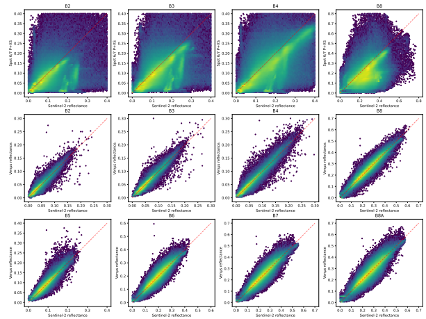
Fig. 2. Scatter plot of pan-sharpened Spot6/7 vs. Sentinel-2 reflectance from sample patches from the Worldstrat dataset (first row) and of Venüs vs. Sentinel-2 reflectance for sample patches from the Sen2Venüs dataset (second and third rows)
