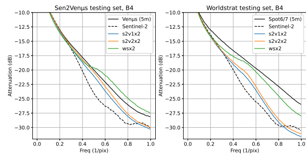
Fig. 19. \mathcal{F}_{AP}^* of SISR model trained on s2v1x2 , s2v2x2 , and wsx2 training sets, with the geom+rad strategy, computed on B4 of Sen2Venus testing set (left) and Worldstrat testing set (right).
