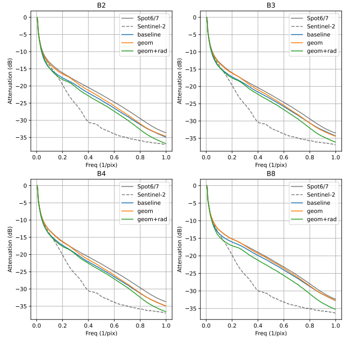
Fig. 33. Frequency Domain Analysis for baseline and proposed robust strategy of the Sen2Venüs, 20 m → 5 m experiment with wsx4 training set, evaluated on the Worldstrat testing set.
