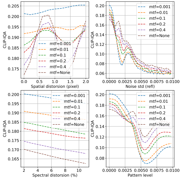
Fig. 25. Benchmarking of CLIP-IQA (lower is better) with respect to geometric distortion, radiometric distortion, noise level and chessboard pattern level, for different level of blur, ranging from mtf=0.4 (very sharp images) to mtf=0.001 (very blurry images)
