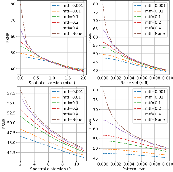
Fig. 4. Benchmarking of PSNR (higher is better) with respect to geometric distortion, radiometric distortion, noise level and chessboard pattern level, for different levels of blur, ranging from mtf=None (no blur applied) or mtf=0.4 (very sharp images) to mtf=0.001 (very blurry images).
