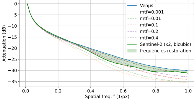
Fig. 8. Normalized log-Frequency Attenuation Profile \mathcal{F}_{AP}^* for reference Venus patches, Sentinel-2 2x bicubic up-sampled, and different levels of blur, for band B2. Spatial frequencies in x axis correspond to normalized spatial frequencies f = \frac{f_n}{f_N} .
