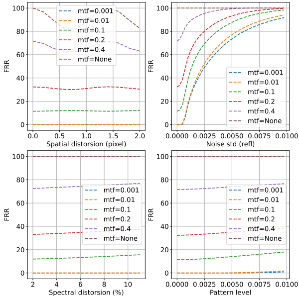
Fig. 10. Benchmarking of the proposed FRR metric (higher is better) with respect to geometric distortion, radiometric distortion, noise level and chessboard pattern level, for different level of blur, ranging from mtf=0.4 (very sharp images) to mtf=0.001 (very blurry images)
