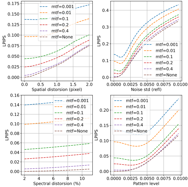
Fig. 6. Benchmarking of LPIPS (lower is better) with respect to geometric distortion, radiometric distortion, noise level and chessboard pattern level, for different levels of blur, ranging from mtf=0.4 (very sharp images) to mtf=0.001 (very blurry images)
