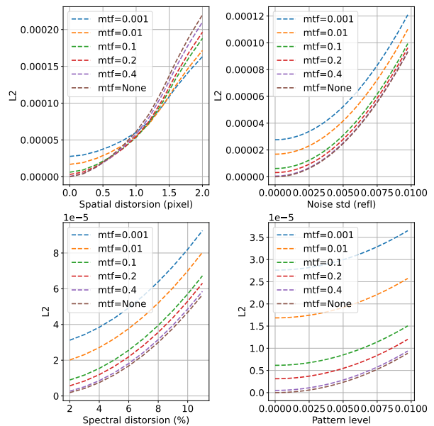
Fig. 23. Benchmarking of RMSE (lower is better) with respect to geometric distortion, radiometric distortion, noise level and chessboard pattern level, for different level of blur, ranging from mtf= None (no blur applied) or mtf=0.4 (very sharp images) to mtf=0.001 (very blurry images)
