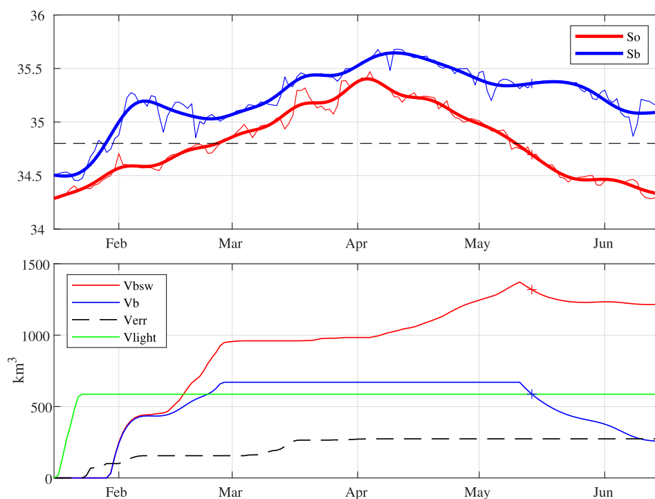
Figure 11. (top) Daily averaged value of near-surface salinity S_o and near-bottom salinity S_b from the mooring, together with their 14 day low-pass filtered counterpart used to run the Brine-enriched Shelf Water (BSW) production model between 16 January and 17 June 2017. (bottom) Volume of BSW produced in the polynya V_{bsw}(t) since 16 January 2017 according to Equation 12 of the box model with linear stratification (red line), which includes the accumulated exported flux and the volume of BSW remaining in the domain V_b(t) according to Equation 11 (blue line). V_{light} is the volume of dense water fresher than 34.8 (green line), thus not identified as BSW. An estimate of the cumulative error V_{err} is also displayed (black dashed line). Units in \text{km}^3 .
