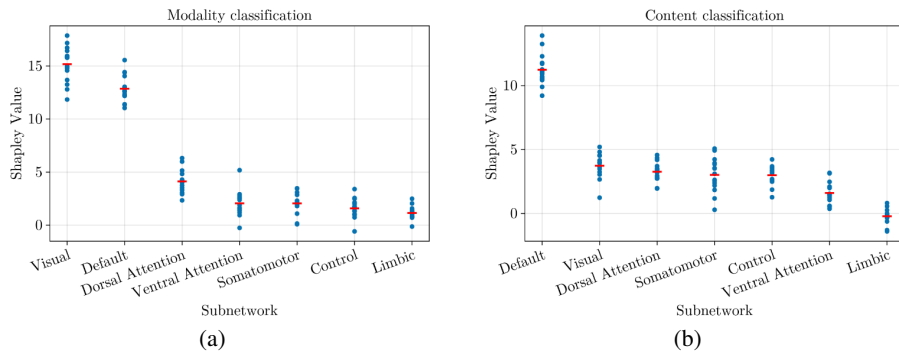
Fig. 1. Distribution of Shapley values for modality classification and content classification.
