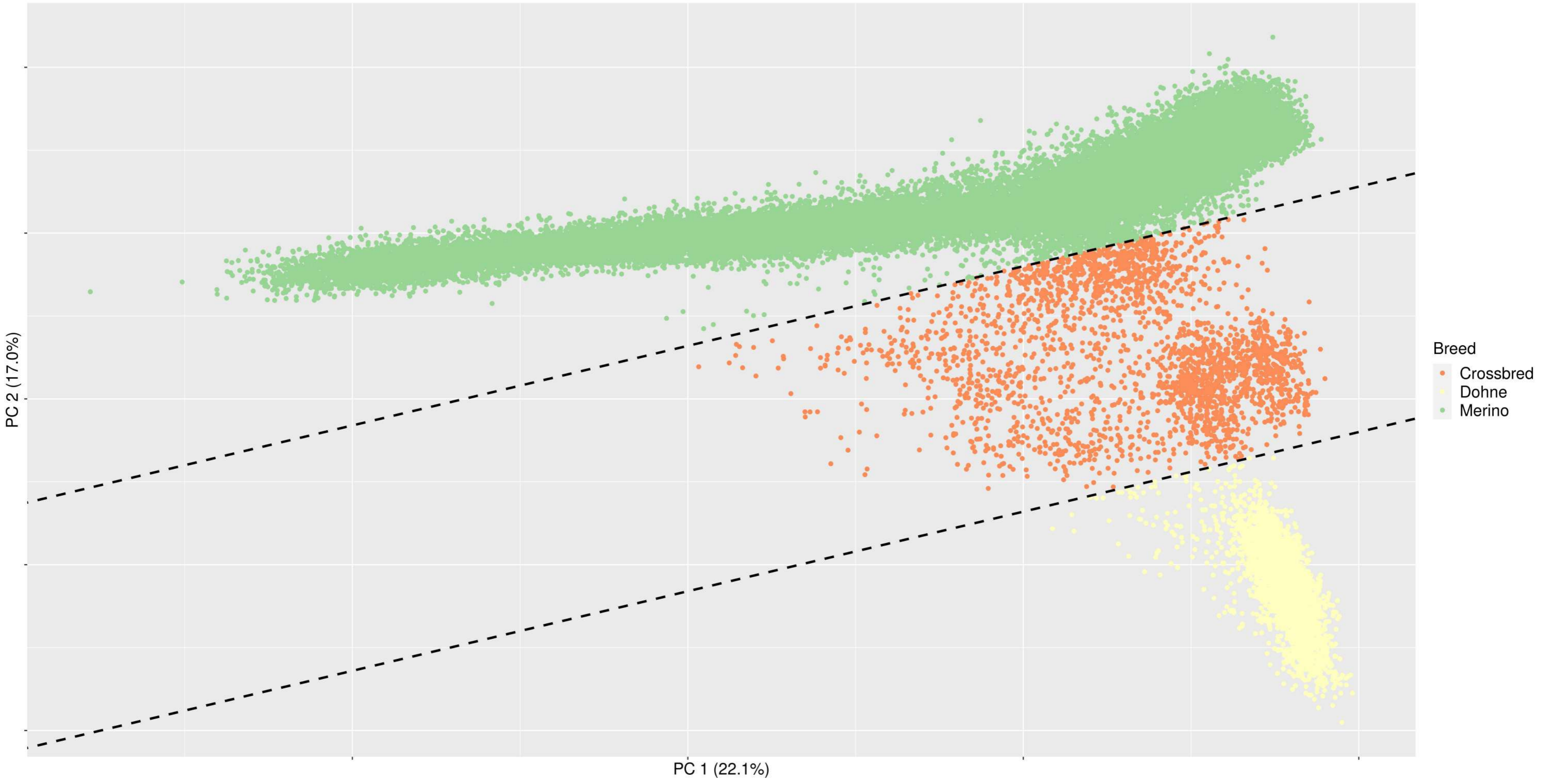
Split of population according to PCA coordinates
