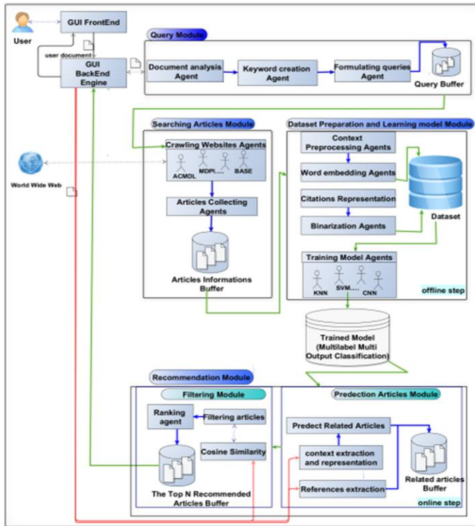
Figure 1. The general architecture of the MASSPR system
