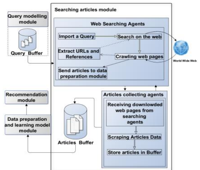
Figure 4. Sub-architecture of the searching articles module
