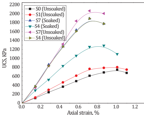
Figure 9. Influence of 5 % CW and 1.5 to 2% OPC on UCS of stabilised soils
