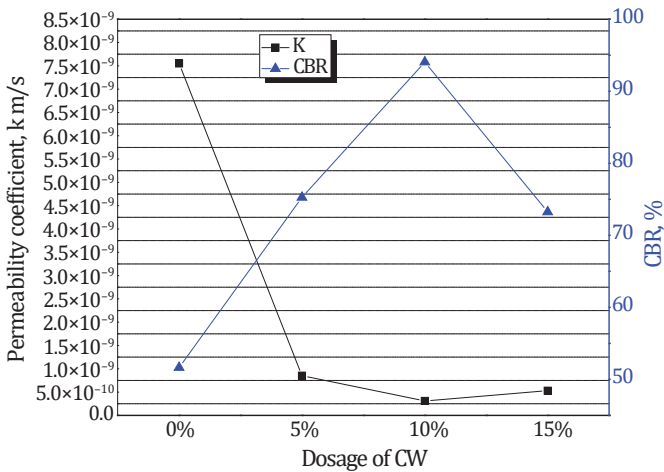
Figure 17. Relationship between permeability and CBR
