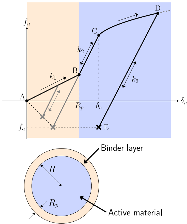
Fig. 1. Normal force f_n as a function of overlap \delta_n and schematic representation of the binder-covered particle model of the electrode. The colored zones represent the contact zones between binder layers and between particles, respectively.
